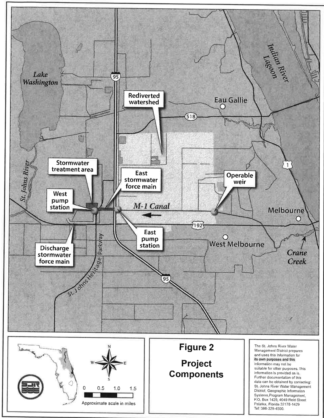
Figure 2. Crane Creek M-1 Canal Flow Restoration Project Components.
