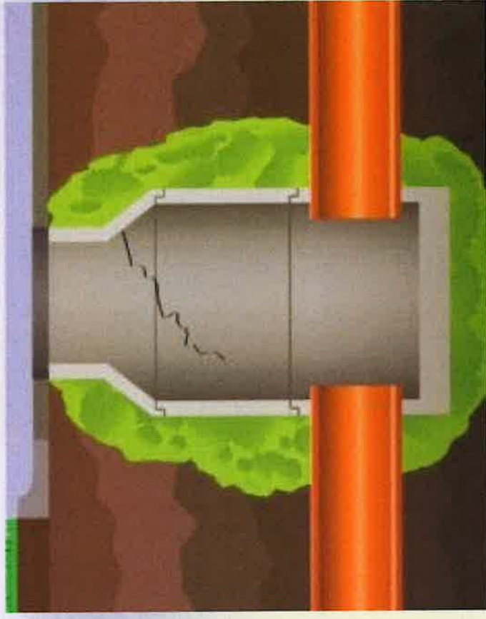
Figure 22 - Manhole Intrusion
