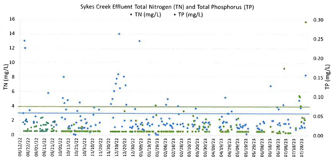
Figure 4-39. Effluent Concentrations from Interstitial Water Treatment at Sykes Creek
