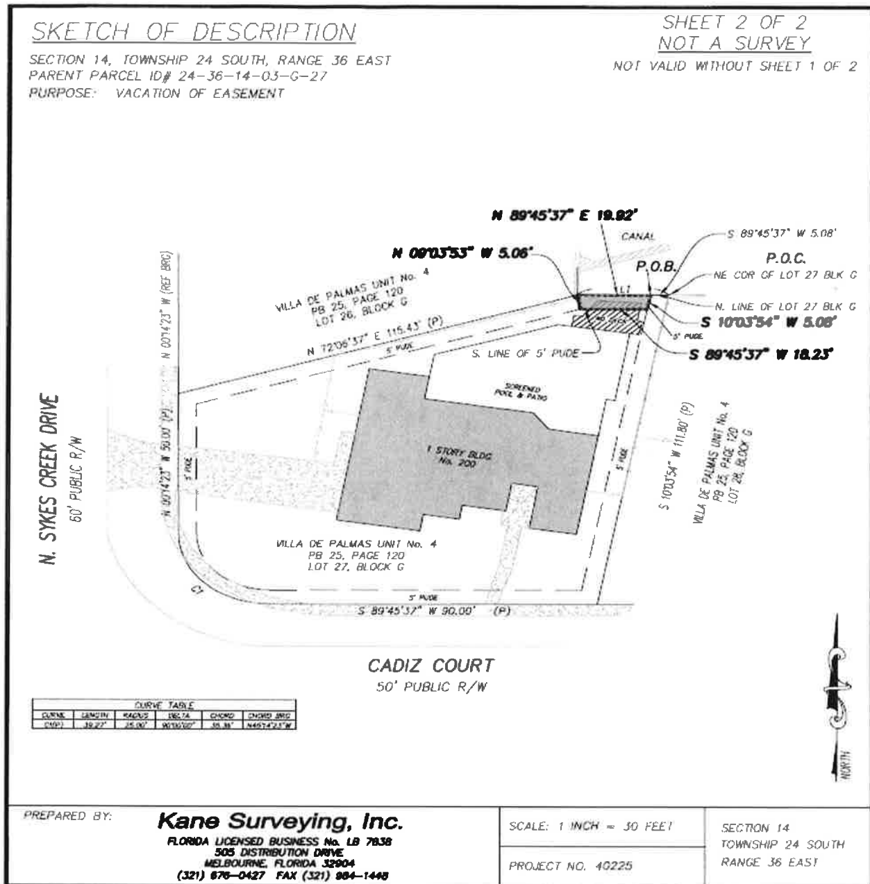
Fig. 6: Sketch of Description. Situated in Section 14, Township 24 South, Range 36 East, Parent Parcel: #24-36-14-03-G-27. Sheet 2 of 2. Not valid without sheet 1 of 2. Sketch illustrate a lot (27) that reside on Cadiz Court, Merritt Island, Florida. A 5-foot public utility & drainage easement lies along the northerly line of lot 27. The coordinates of the area depicted is as follows moving North to East clockwise. North boundary – North 72°06'37" East 115.43'; East boundary South 10°03'54" West 111.80', South boundary – South 89°45'37" West 90.00'. Prepared by: Kane Surveying, Inc., FL LB# 7838. Project NO: 40225.
