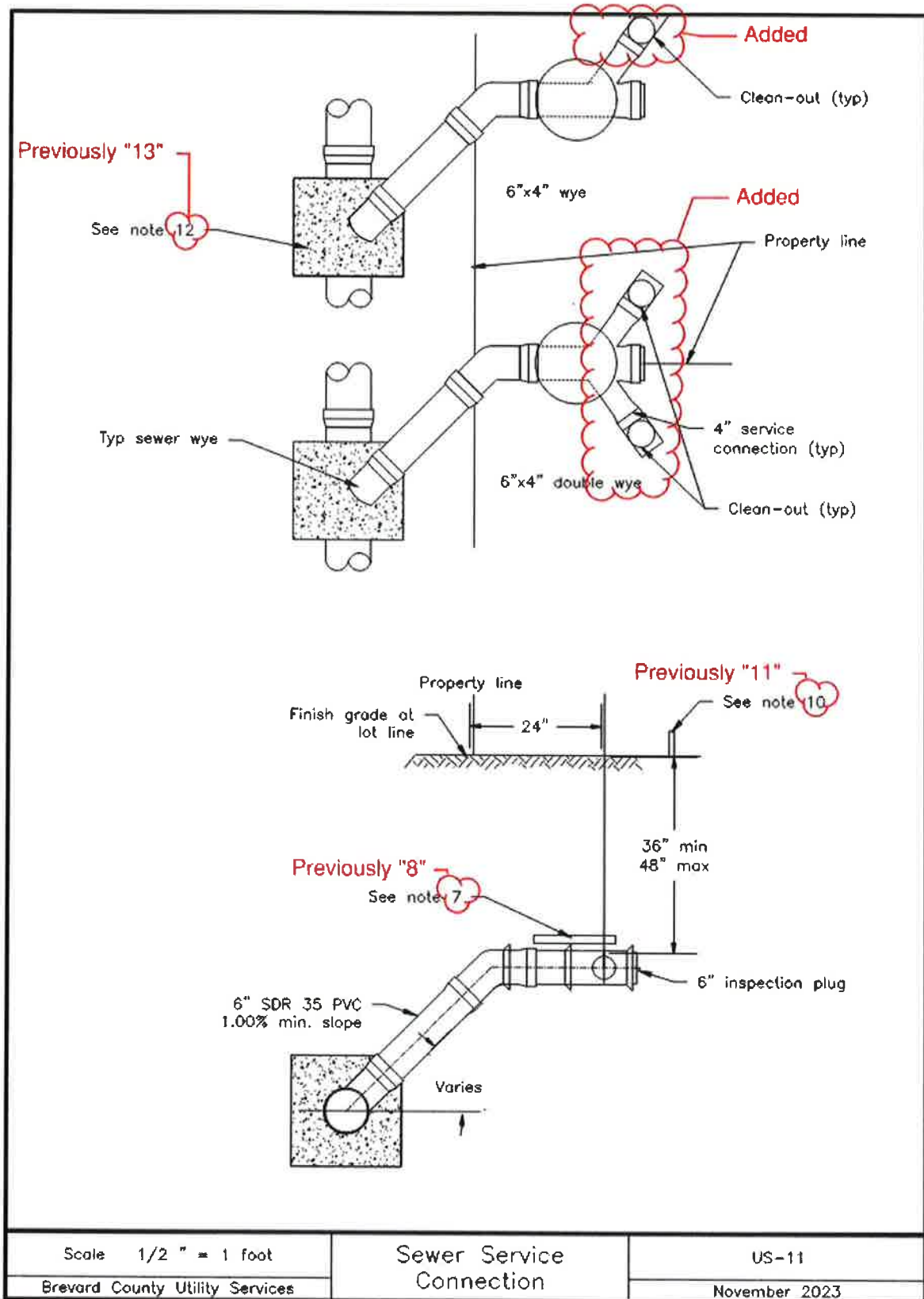
Figure 2 - Sewer Service Connection Details (US-11)
