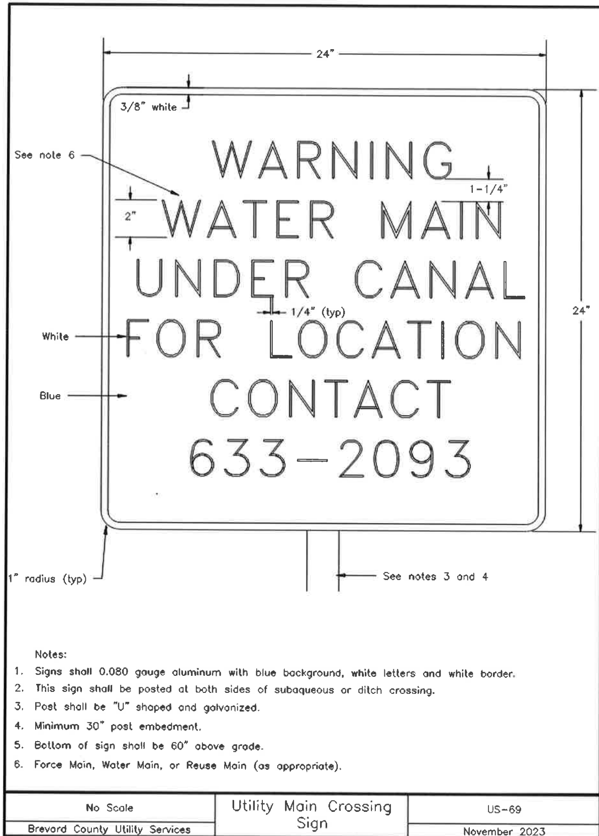
Image Description US-69 Utility Main Crossing Sign
