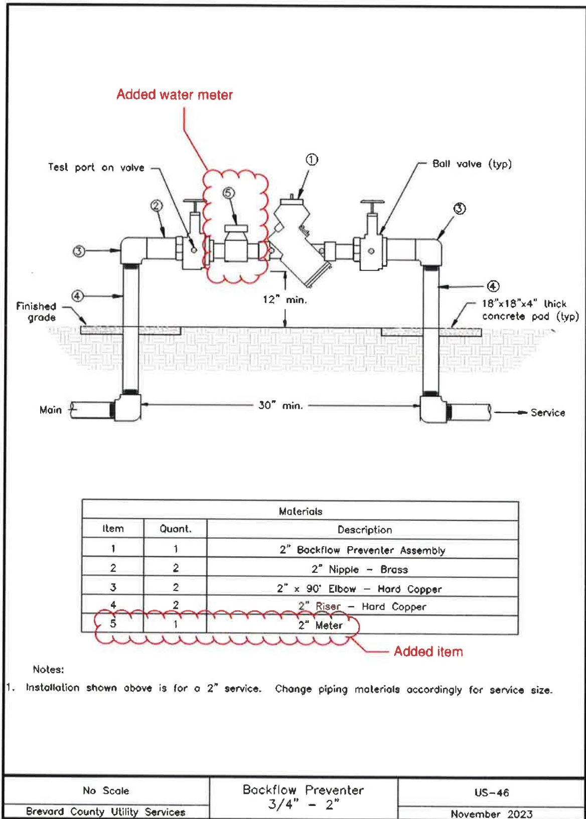
Image Description US-46 Backflow Preventer 3/4" - 2"
