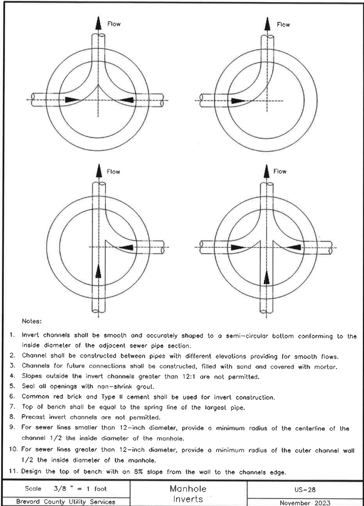
Image Description US-28 -Manhole Inverts
