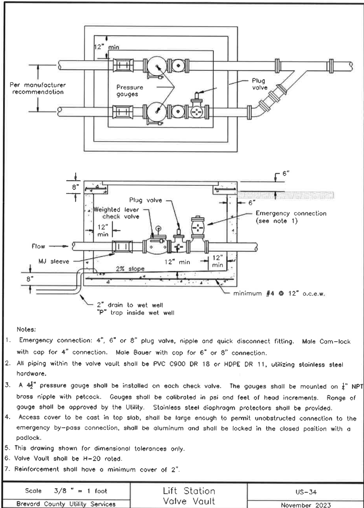
Image Description US-34 Lift Station Valve Vault
