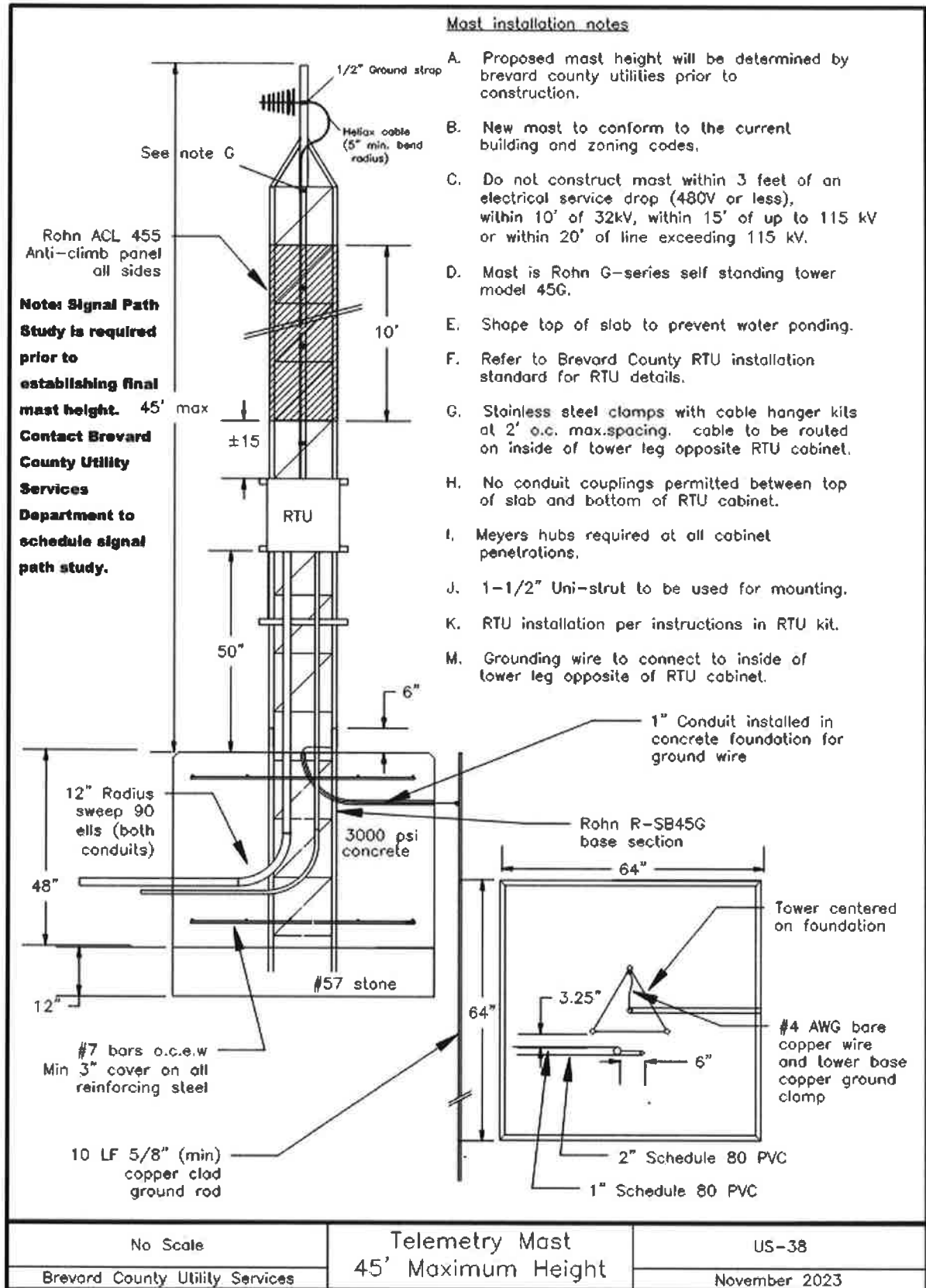
Image Description US-38 Telemetry Mast 45' Maximum Height
