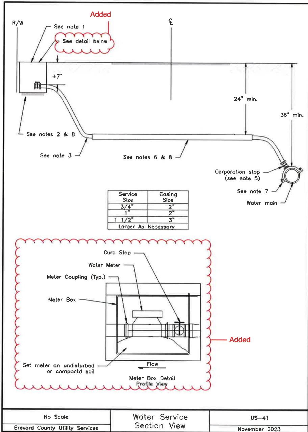
Image Description US-41 Water Service Section View
