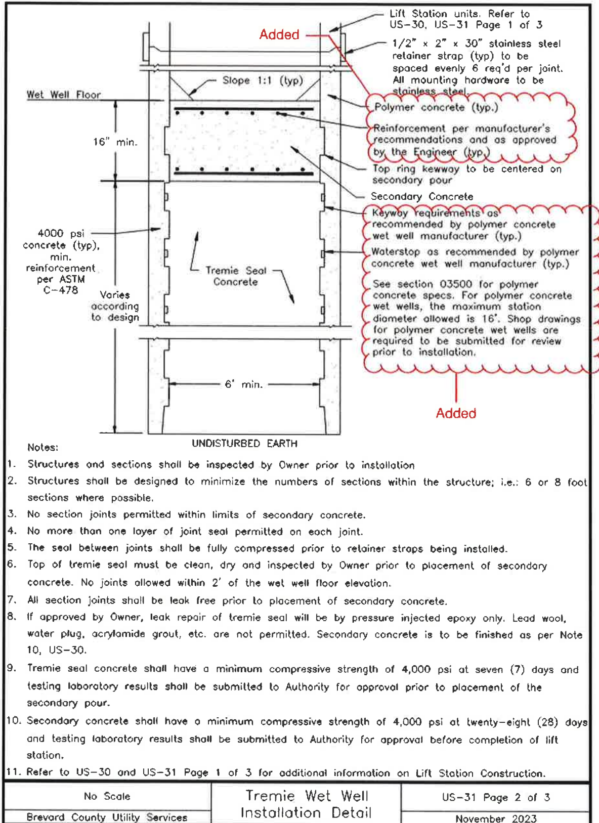
Figure 22 - Tremie Wet Well Installation Detail (US-31 Page 2 of 3)
