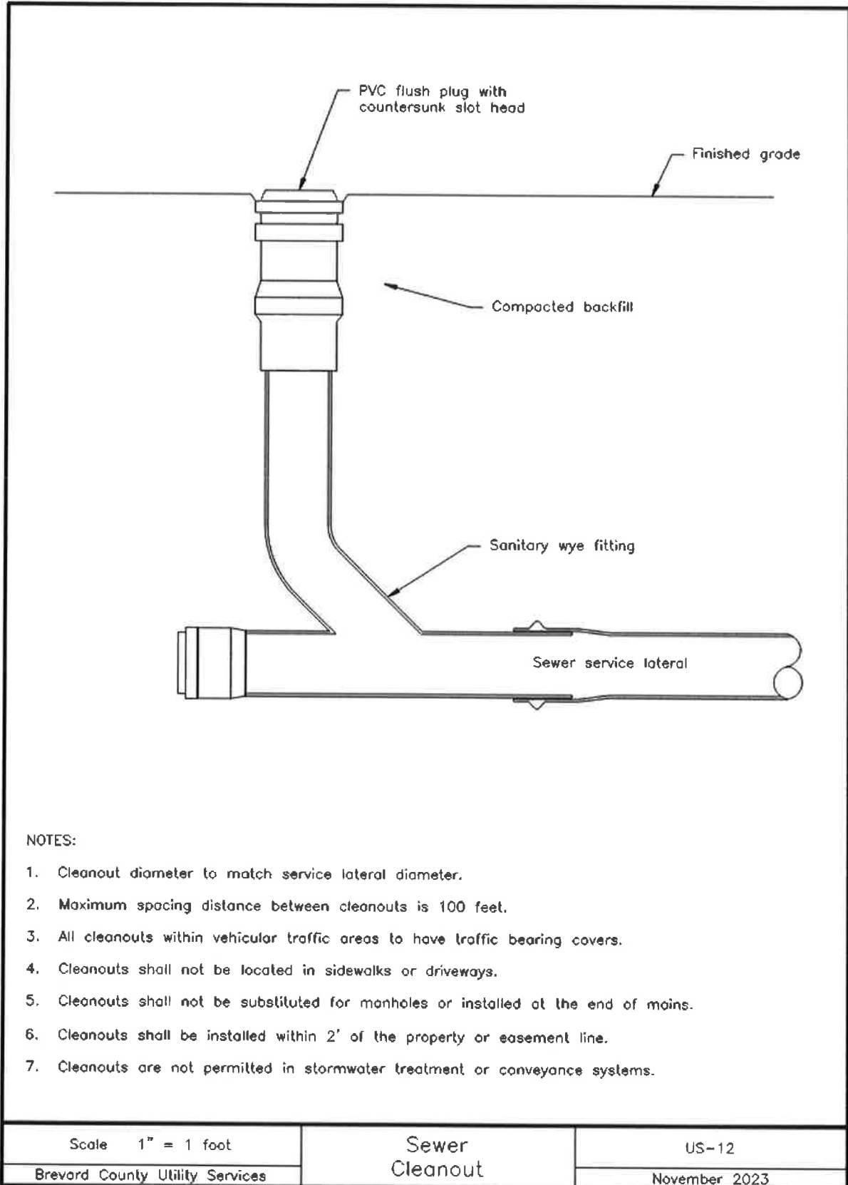
Image Description US-12 Sewer Cleanout
