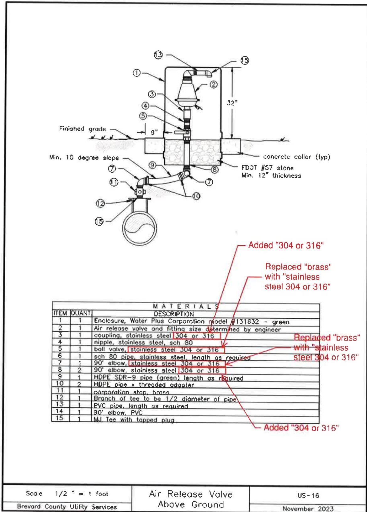
Image Description US-16 Above Ground Air Release Valve
