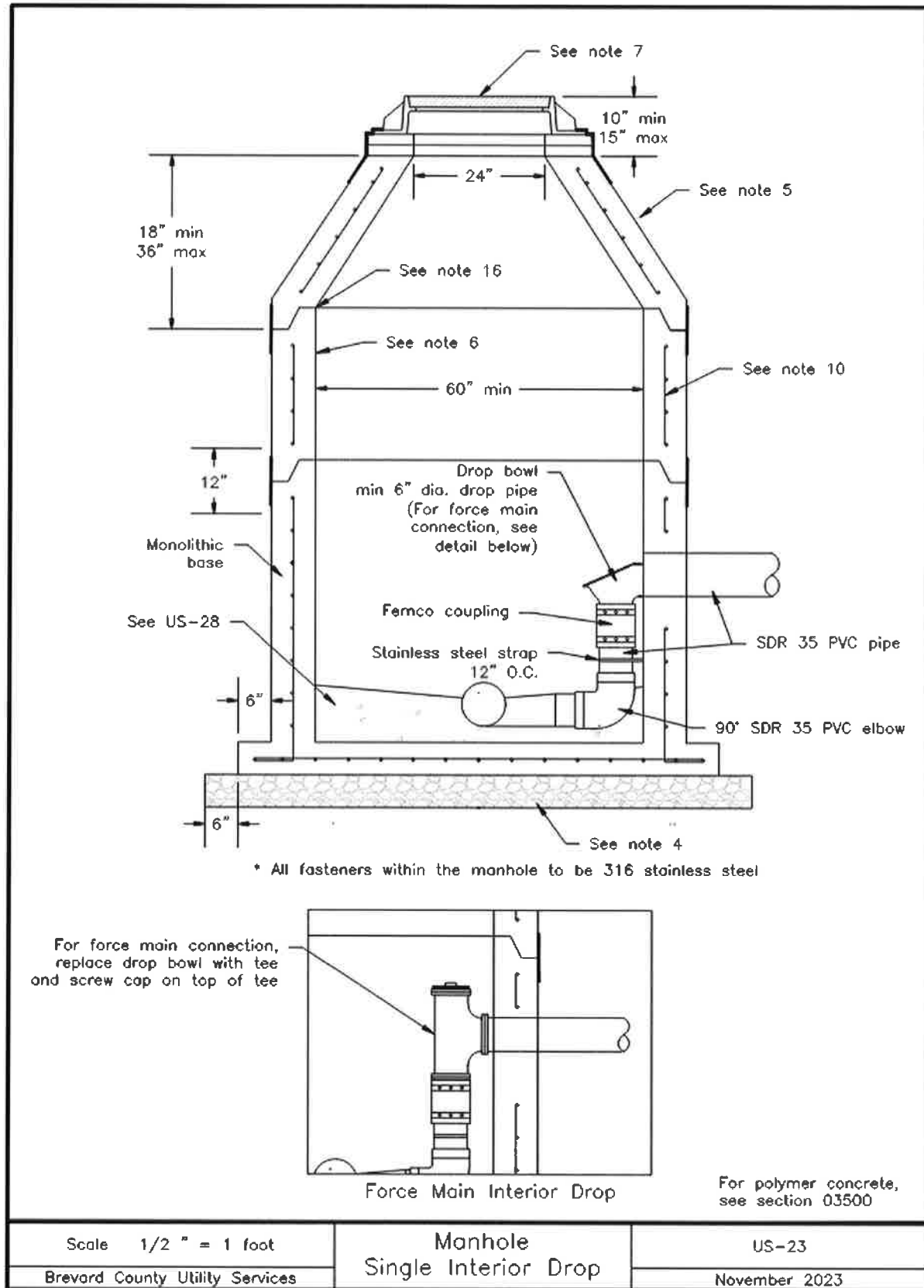
Image Description US-23 – Single Interior Drop Manhole
