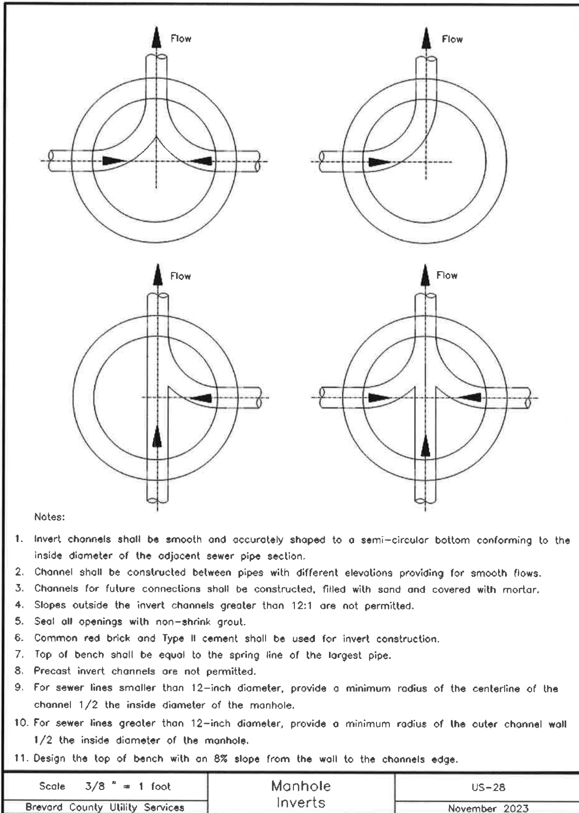
Image Description US-28 -Manhole Inverts
