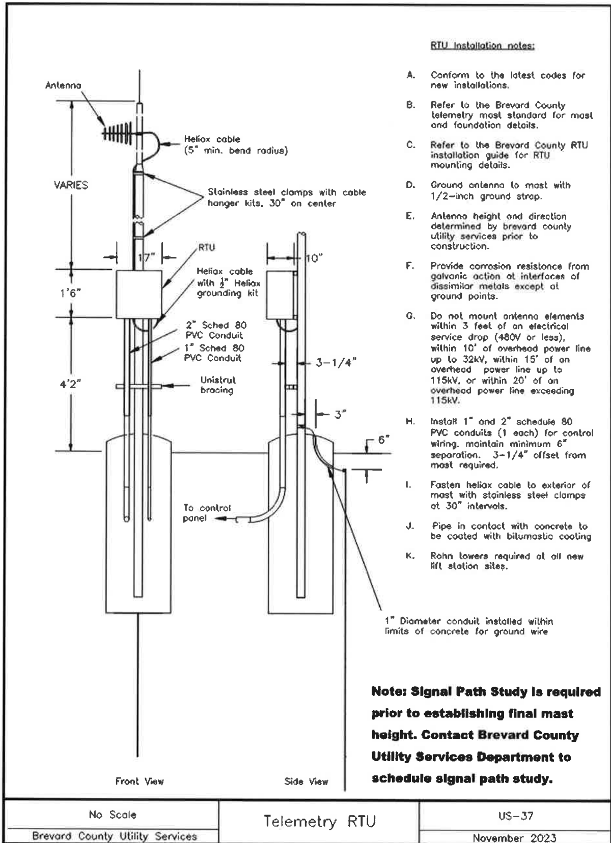
Image Description US-37 Telemetry RTU
