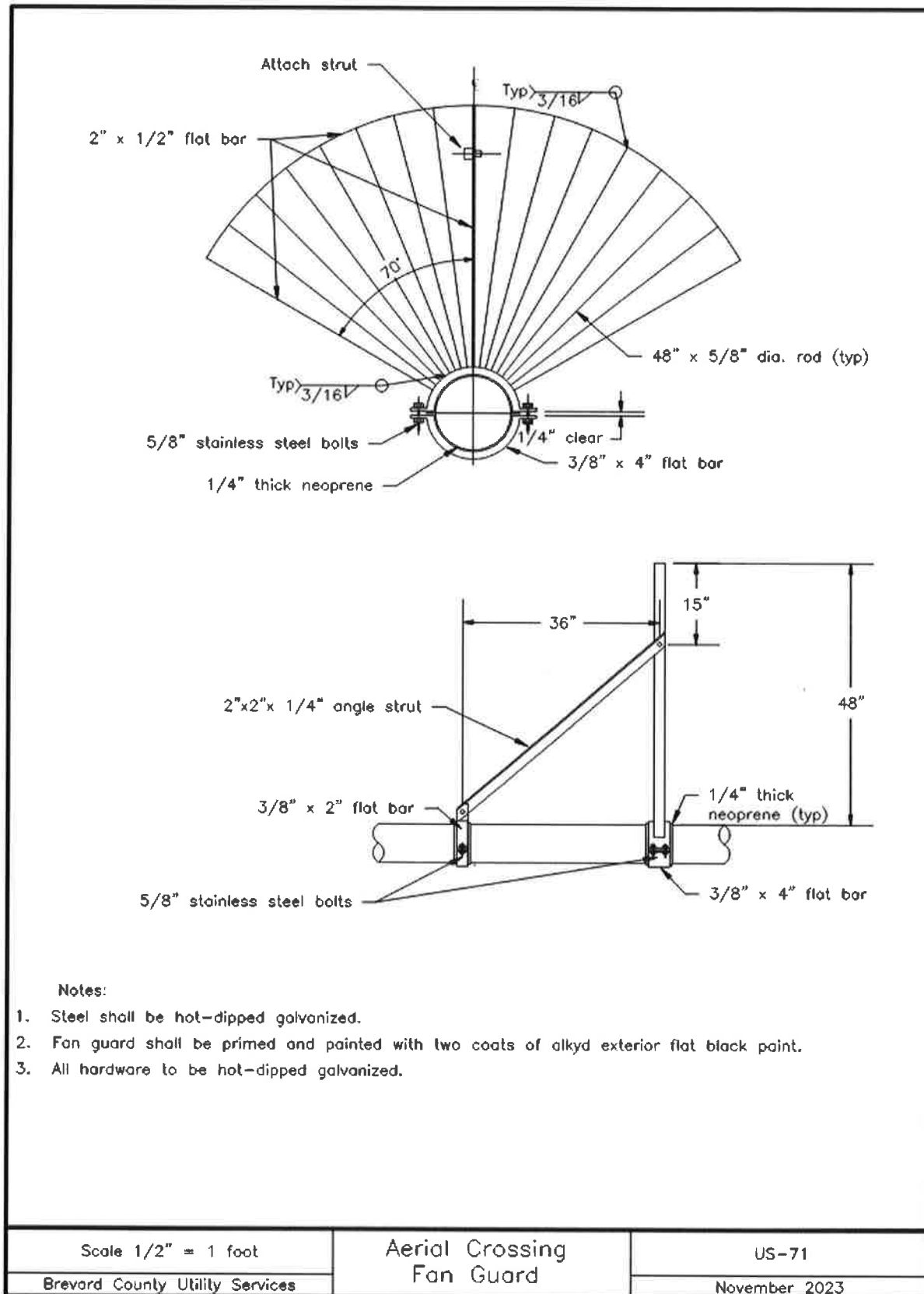
Image Description US-71 Aerial Crossing Fan Guard
