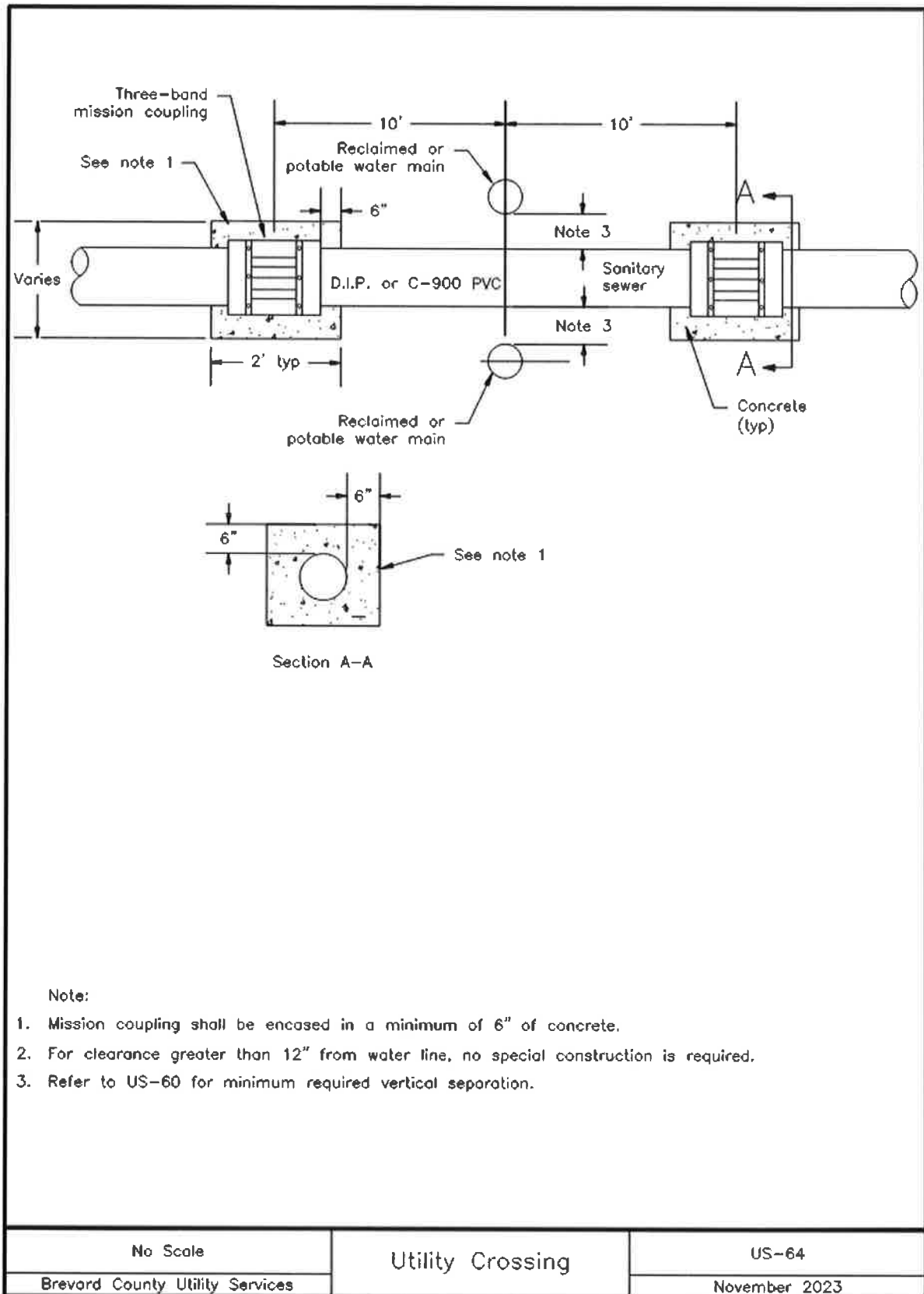
Image Description US-64 Utility Crossing
