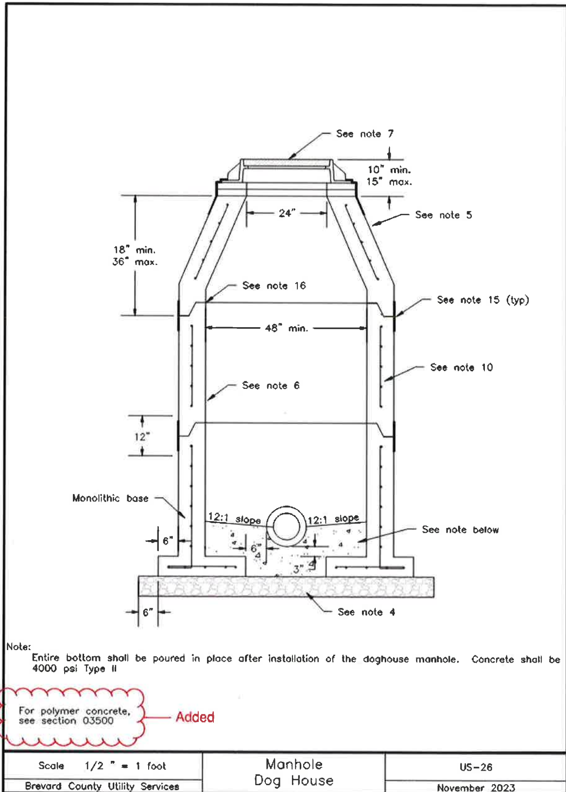
Image Description US-26 – Dog House Manhole
