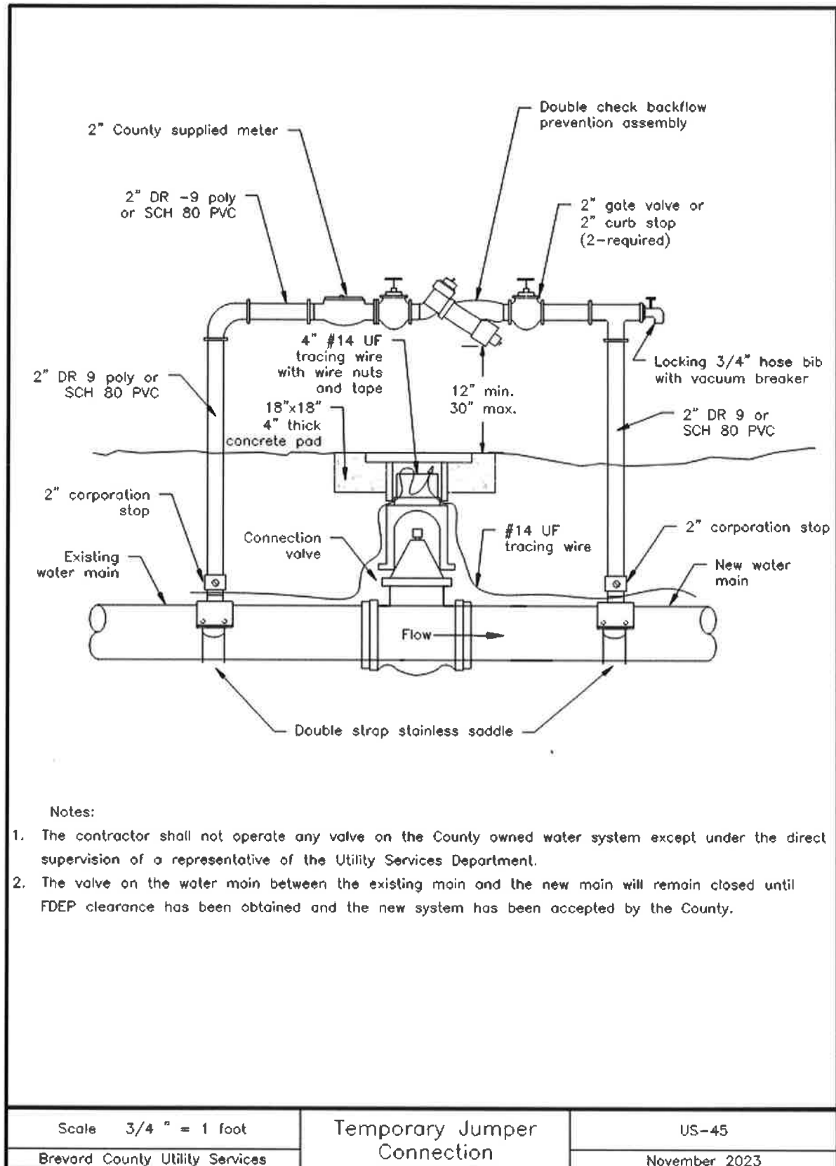
Image Description US-45 Temporary Jumper Connection
