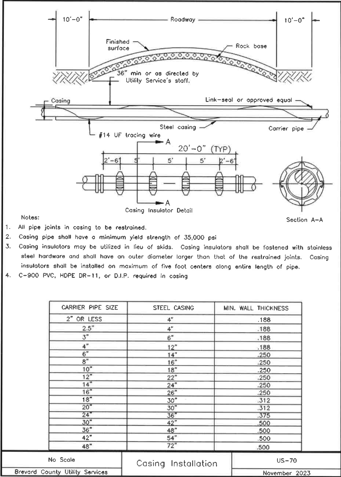
Image Description US-70 Casing Installation
