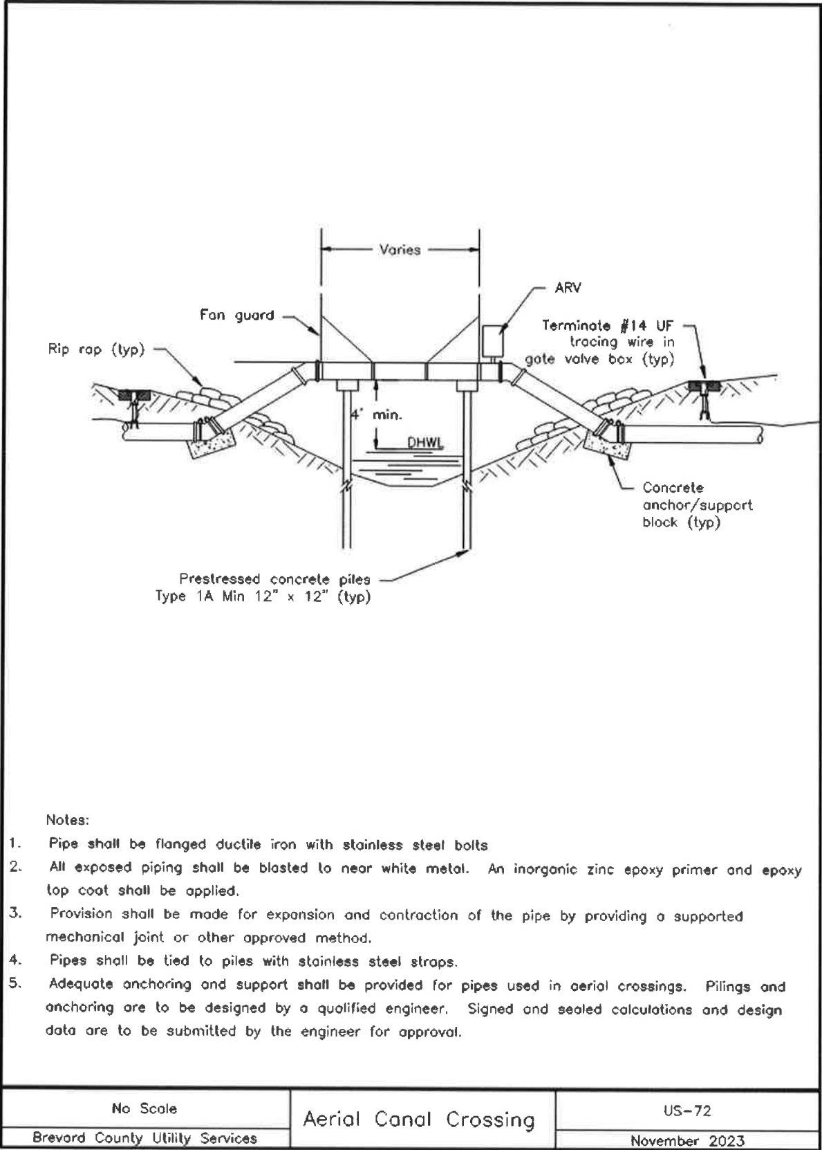
Image Description US-72 Aerial Canal Crossing
