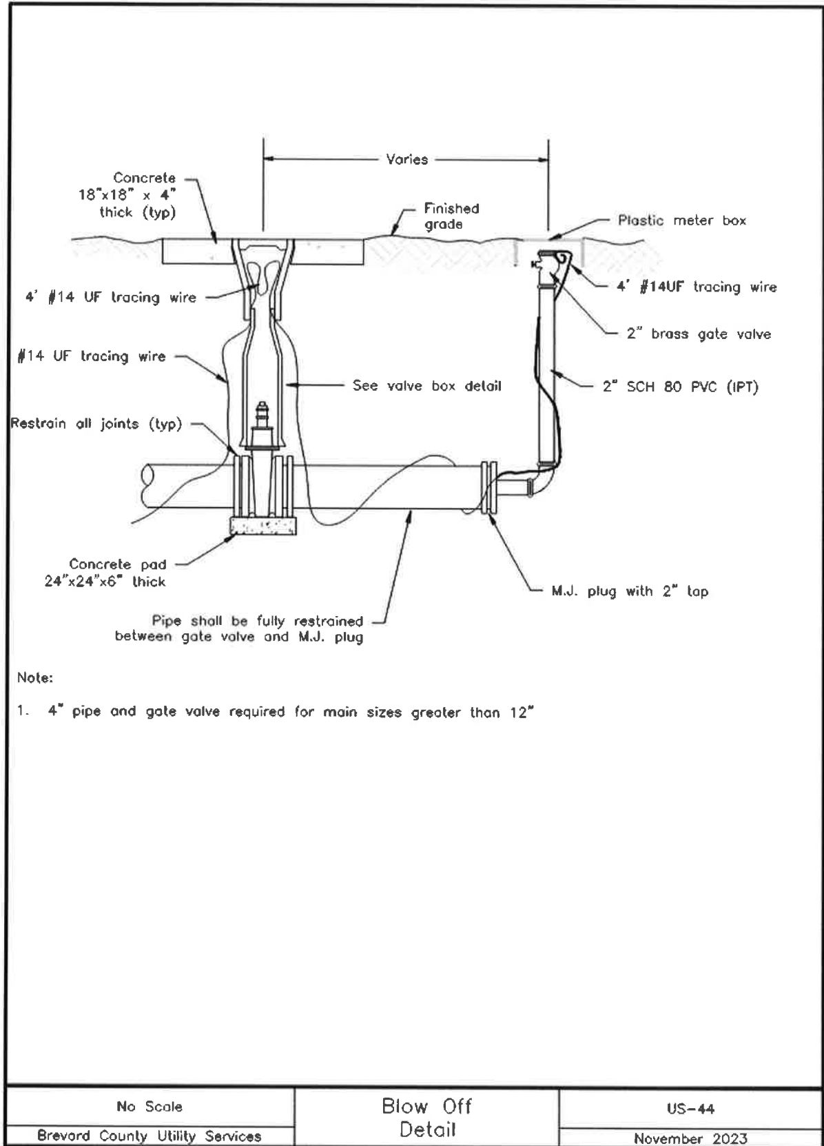
Image Description US-44 Blow Off Detail
