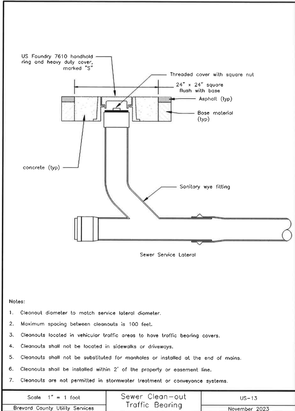
Image Description US-13 Traffic Bearing Sewer Clean-out
