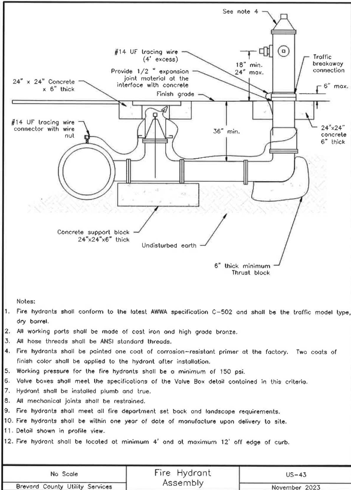
Image Description US-43 Fire Hydrant Assembly
