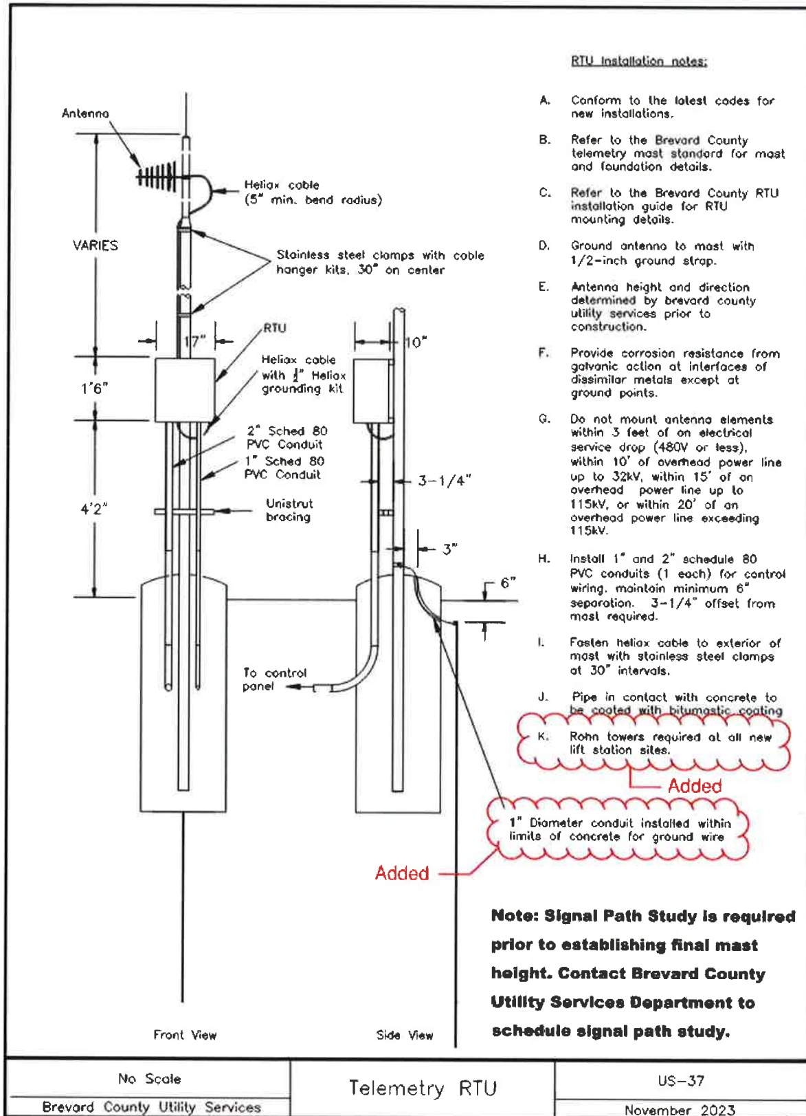
Figure 32 - Telemetry RTU Detail (US-37)
