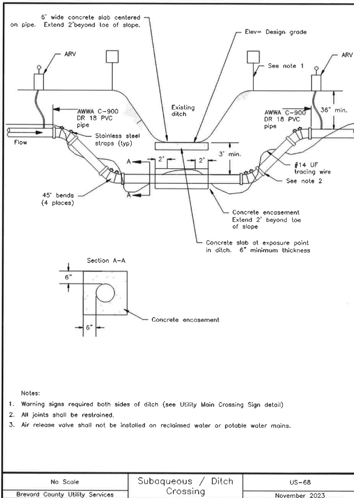
Figure 56 - Subaqueous / Ditch Crossing Detail (US-68)
