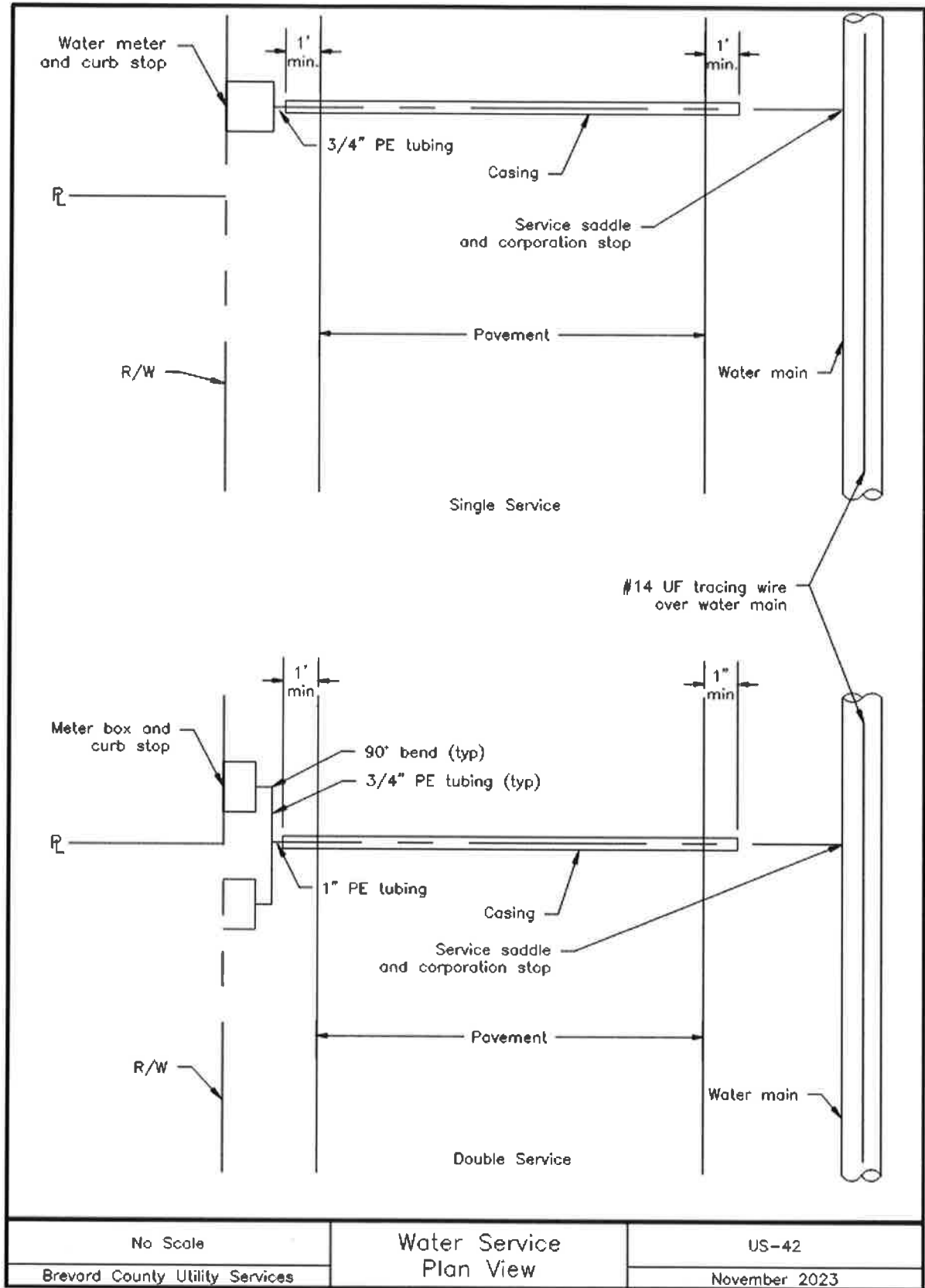
Image Description US-42 Water Service Plan View
