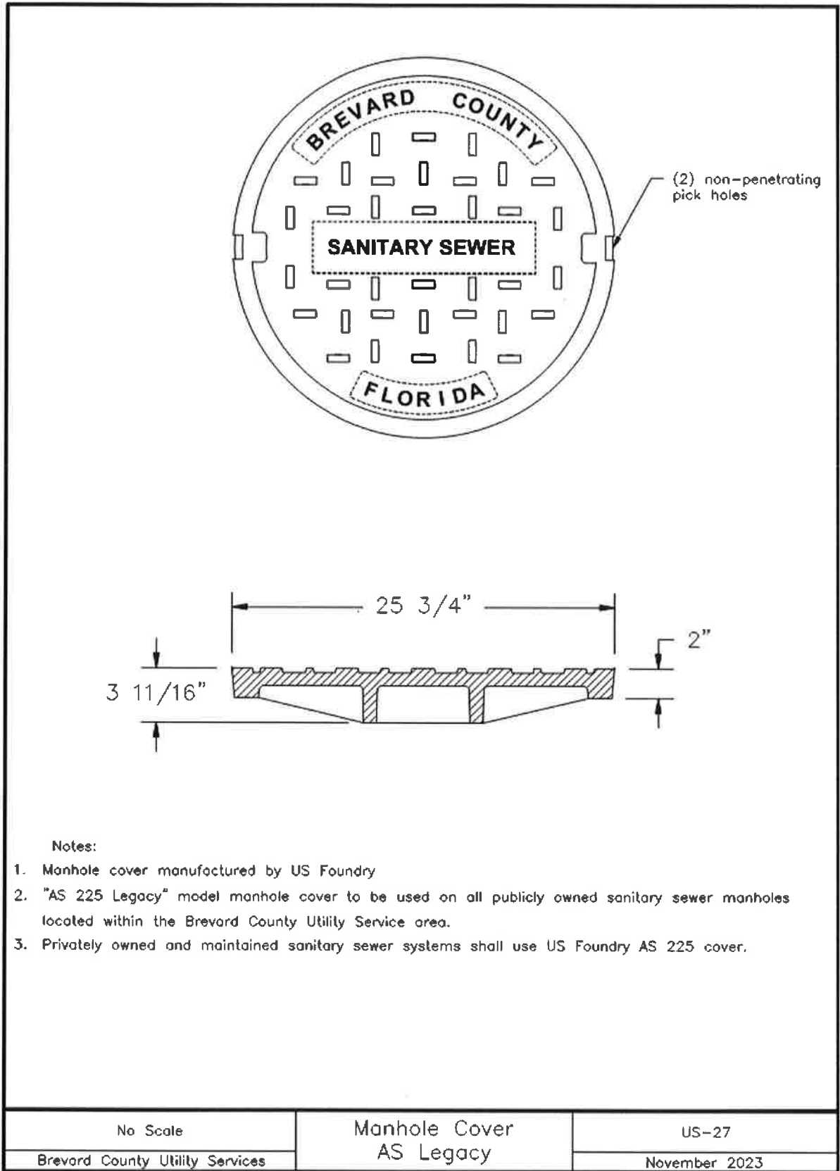
Image Description US-27 -AS Legacy Manhole Cover
