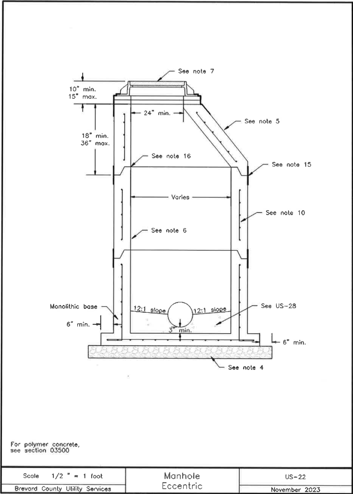
Image Description US-22 – Eccentric Manhole
