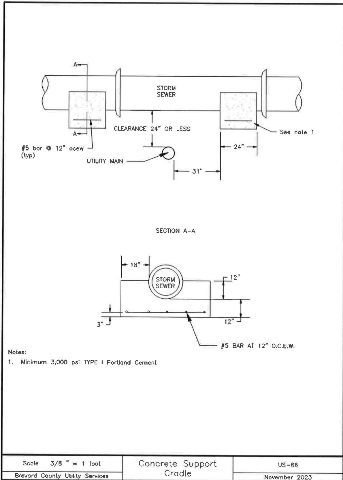
Image Description US-66 Concrete Support Cradle
