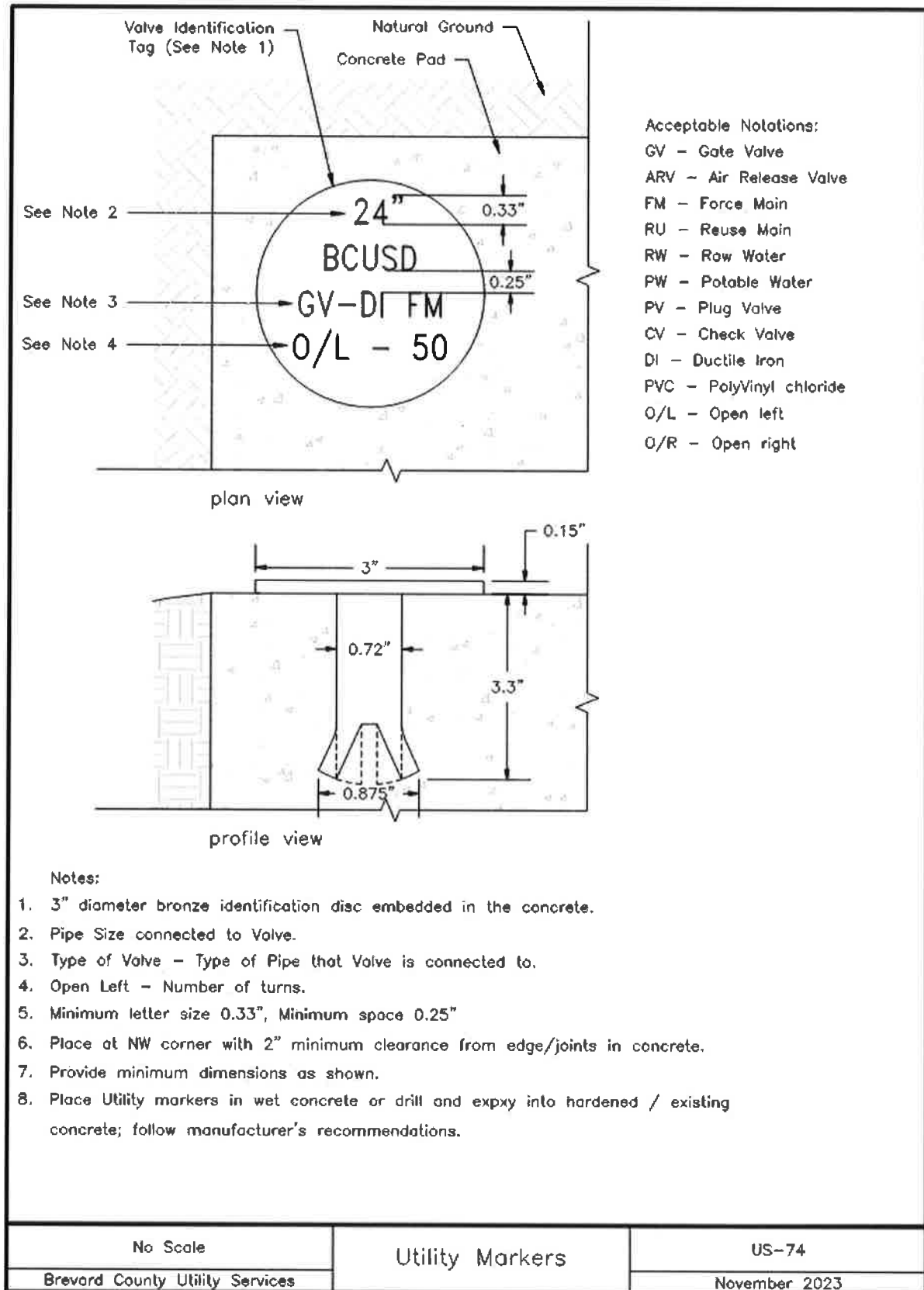
Image Description US-74 Utility Markers
