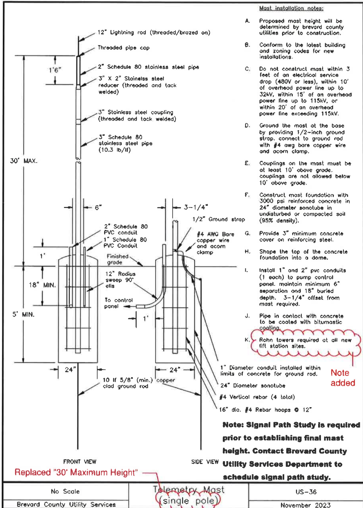
Image Description US-36 Telemetry Mast (single pole)
