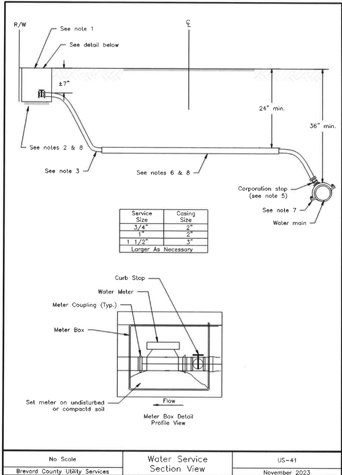
Image Description US-41 Water Service Section View
