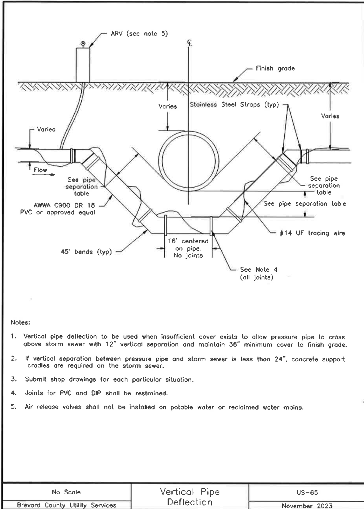
Image Description US-65 Vertical Pipe Deflection
