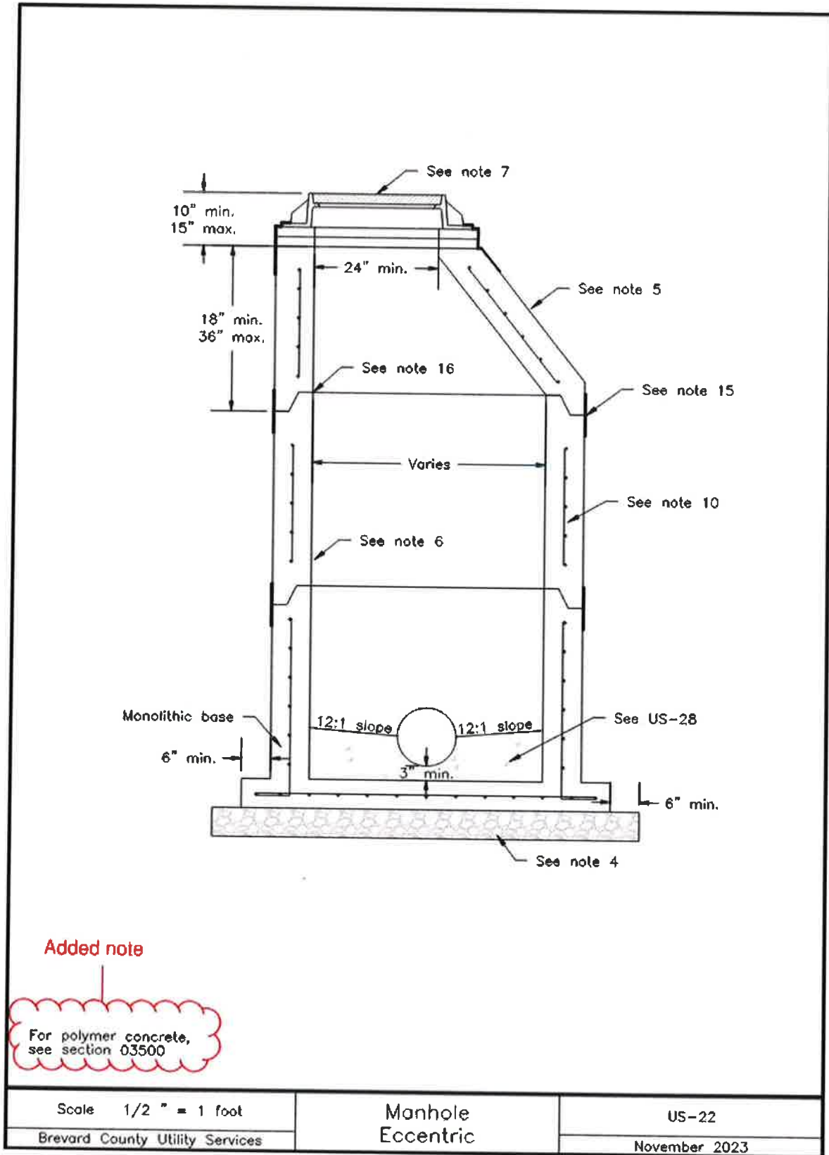
Image Description US-22 – Eccentric Manhole
