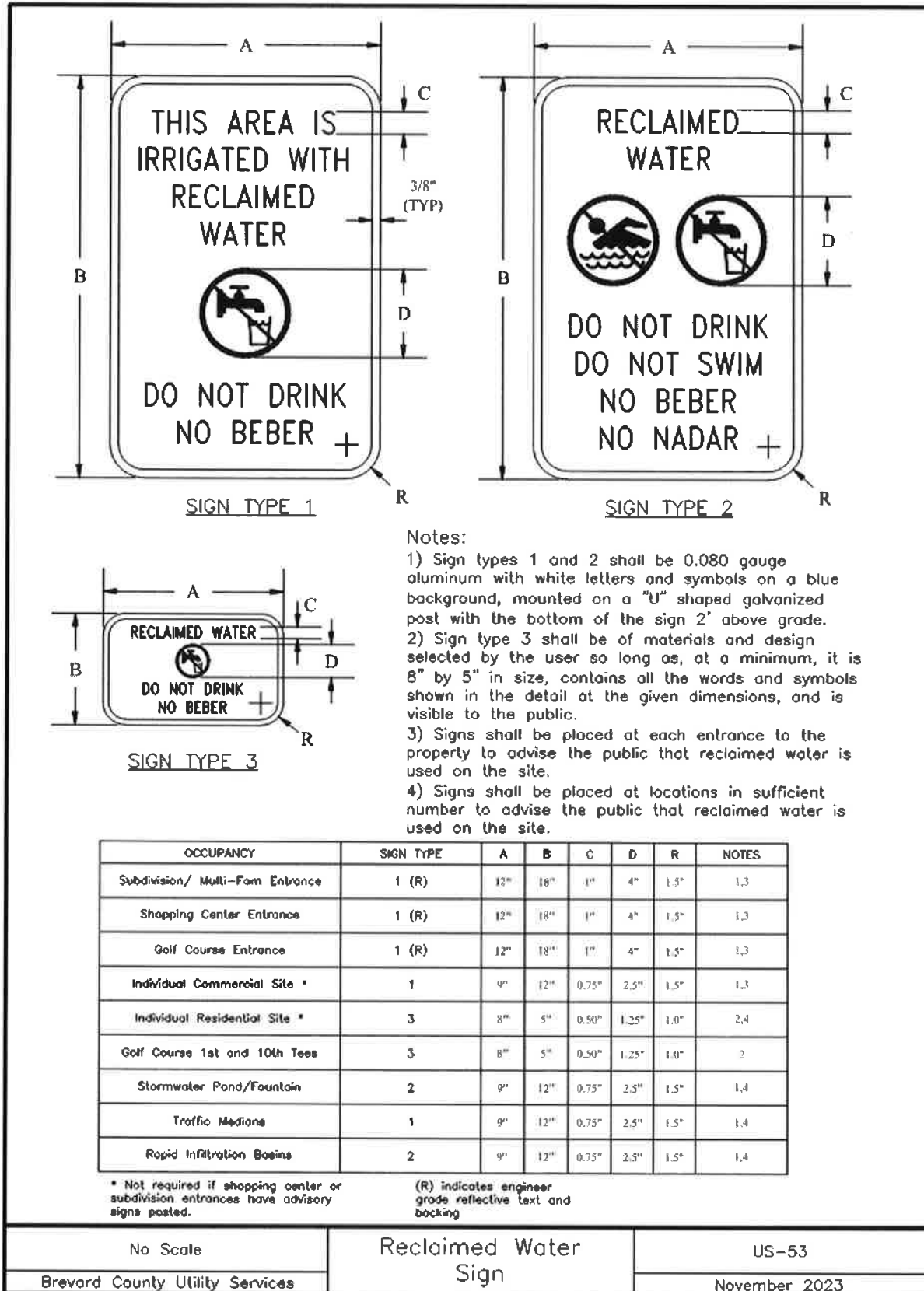
Image Description US-53 Reclaimed Water Sign
