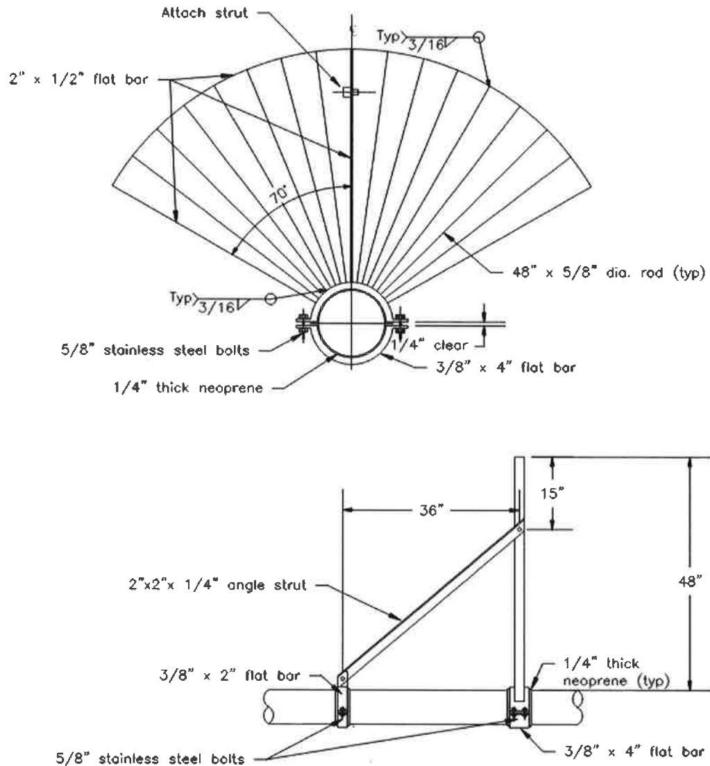
Figure 59 - Aerial Crossing Fan Guard Detail (US-71)
