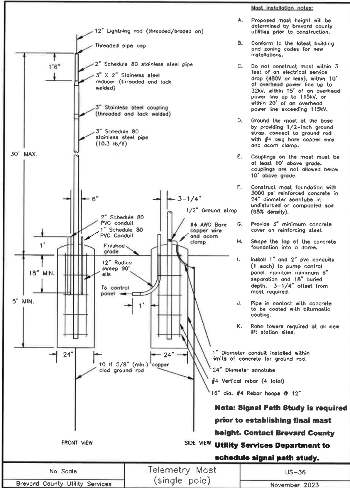
Image Description US-36 Telemetry Mast (single pole)
