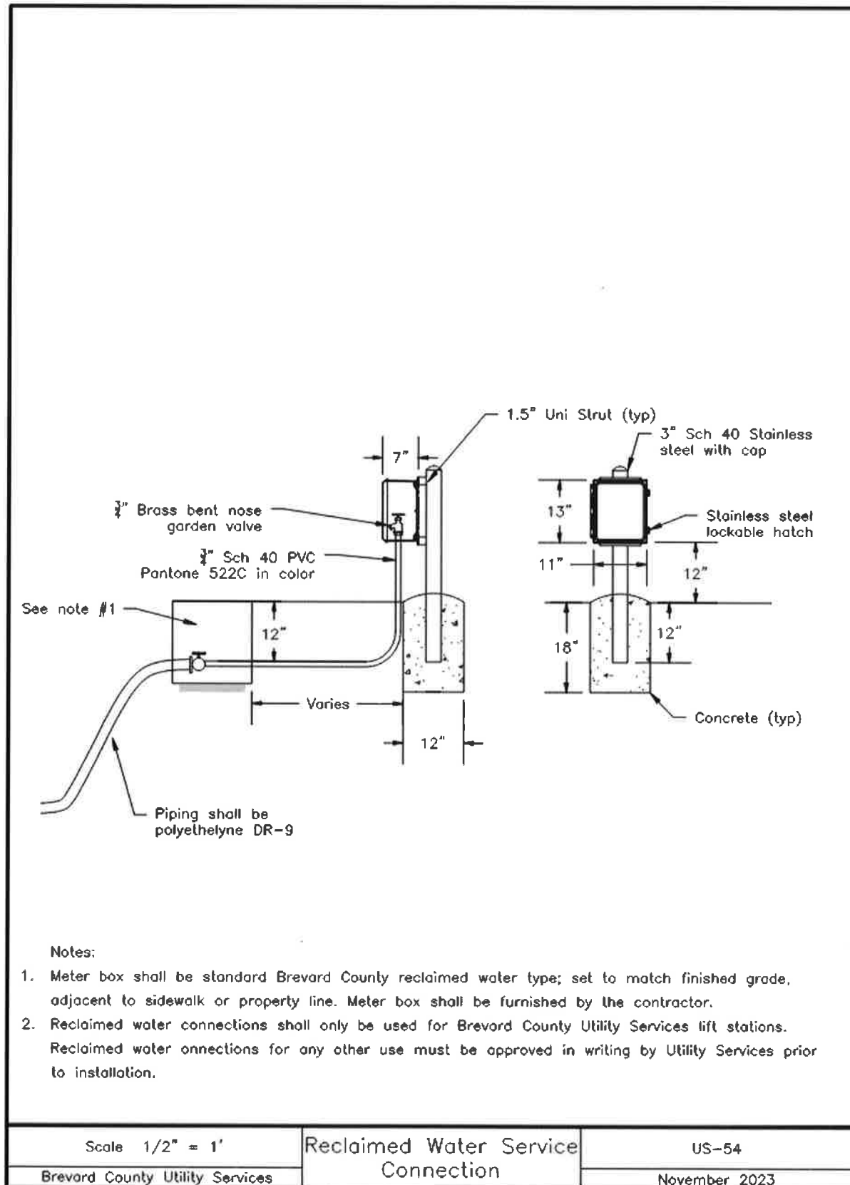
Image Description US-54 Reclaimed Water Service Connection
