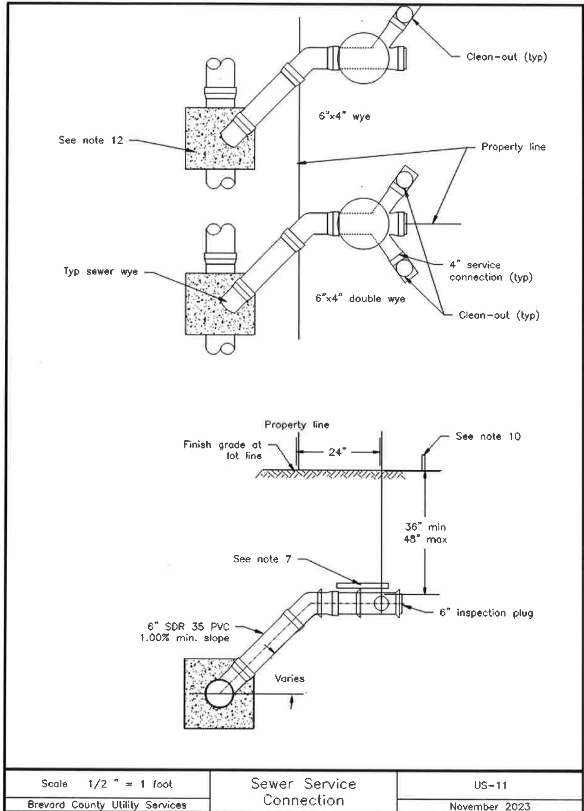
Image Description US-11 Sewer Service Connection
