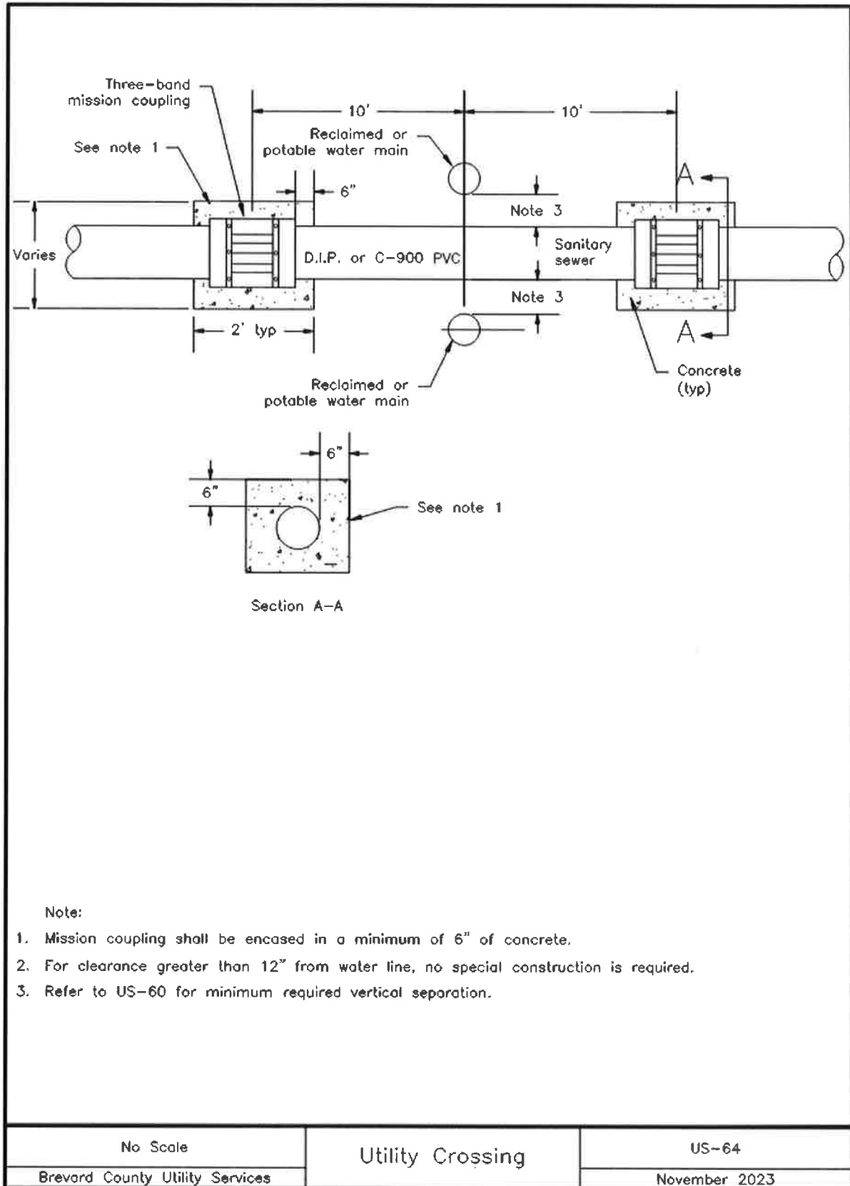
Figure 52 - Utility Crossing Detail (US-64)
