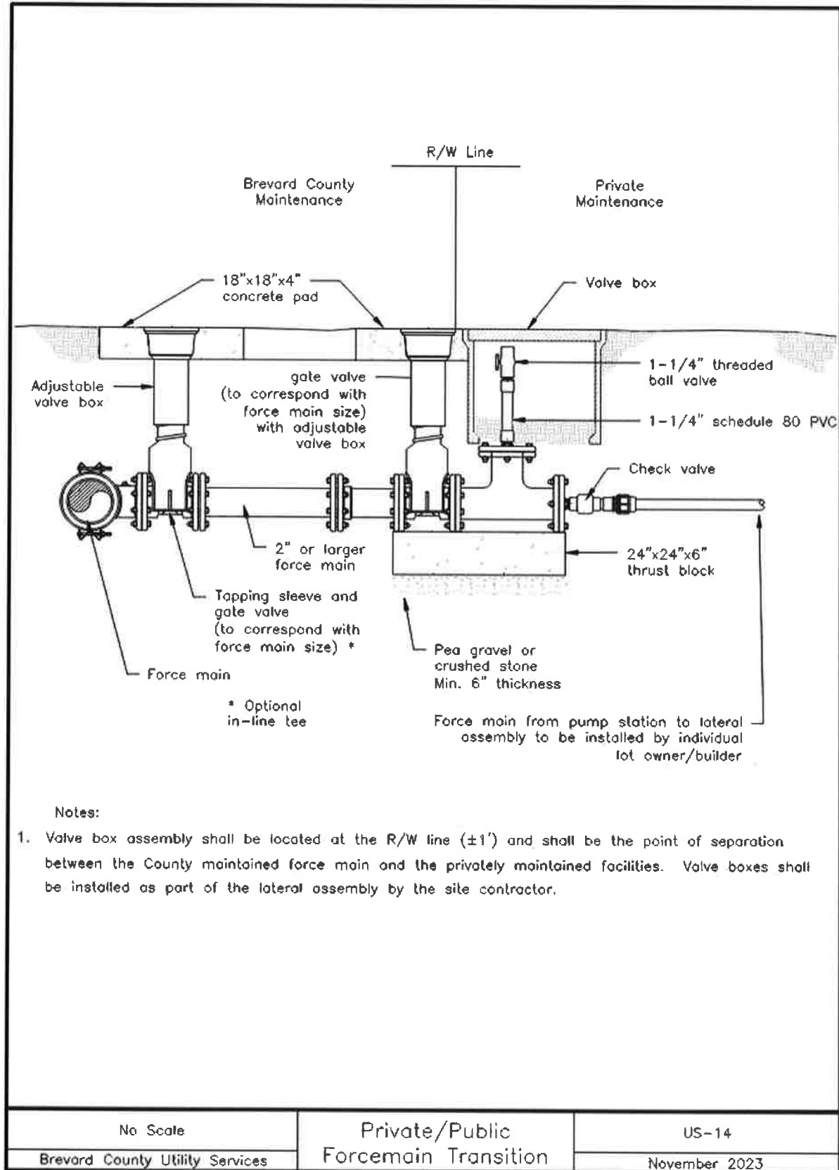
Image Description US-14 Private/Public Force main Transition
