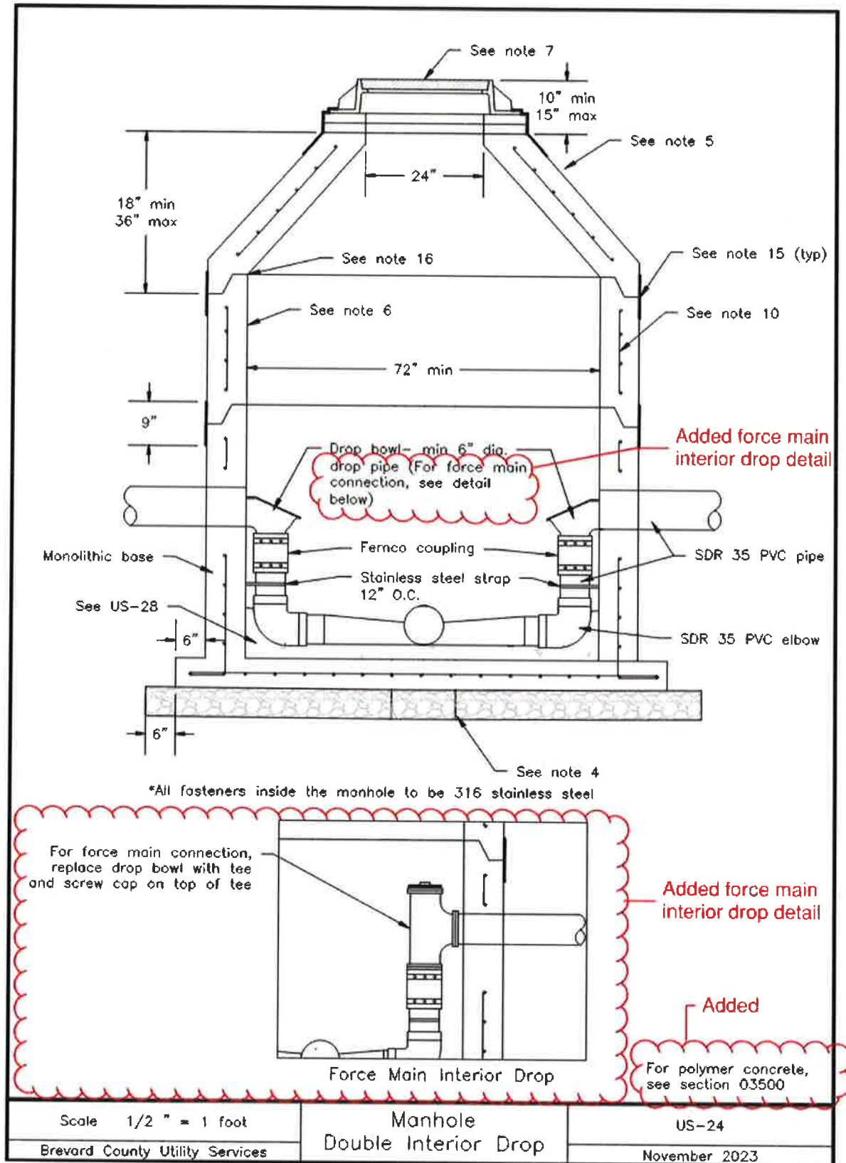
Image Description US-24 -Double Interior Drop Manhole
