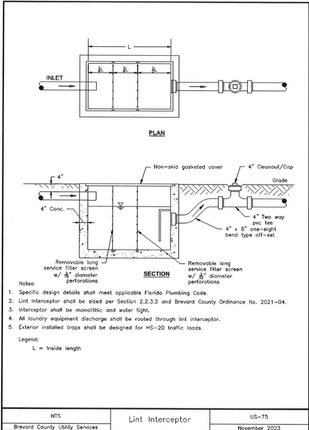
Image Description US-75 Lint Interceptor
