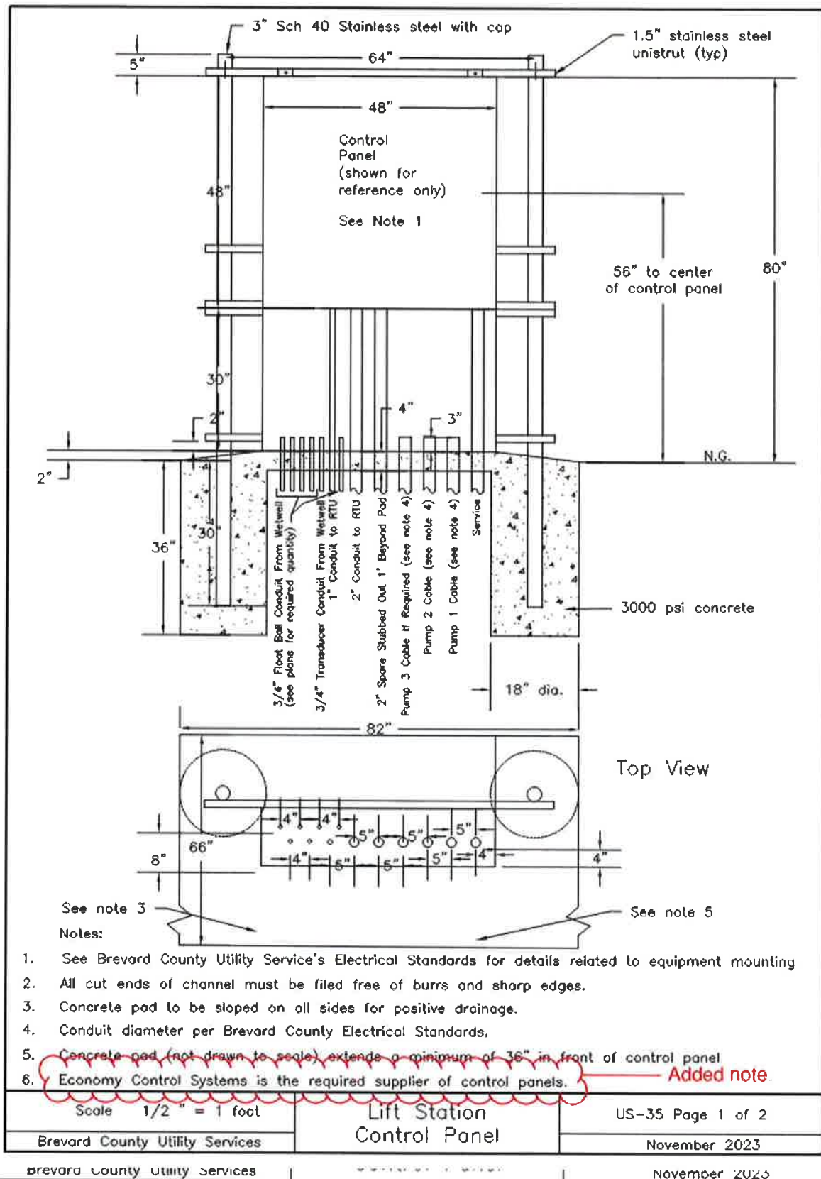
Image Description US-35 Page 1 of 2 (Elec-10-ALL) Lift Station Control Panel
