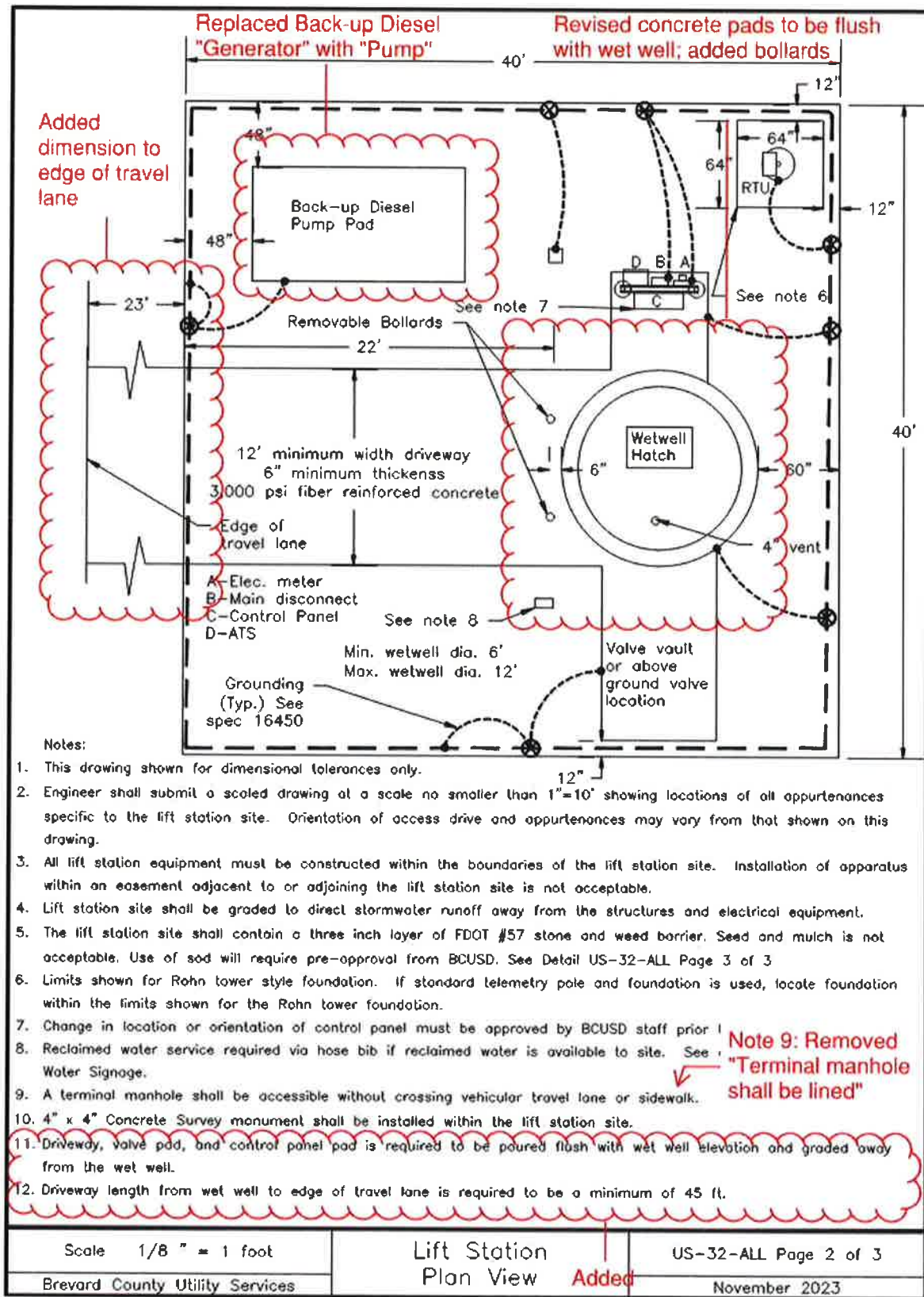
Image Description US-32-ALL Page 2 of 3 Lift Station Plan View
