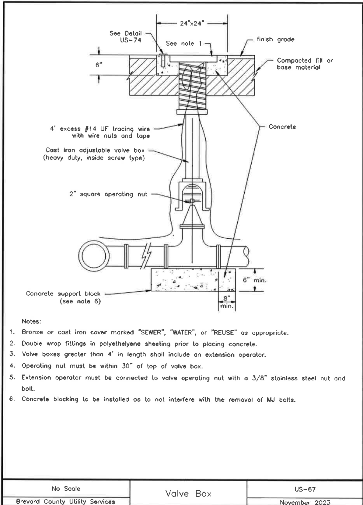
Image Description US-67 Valve Box
