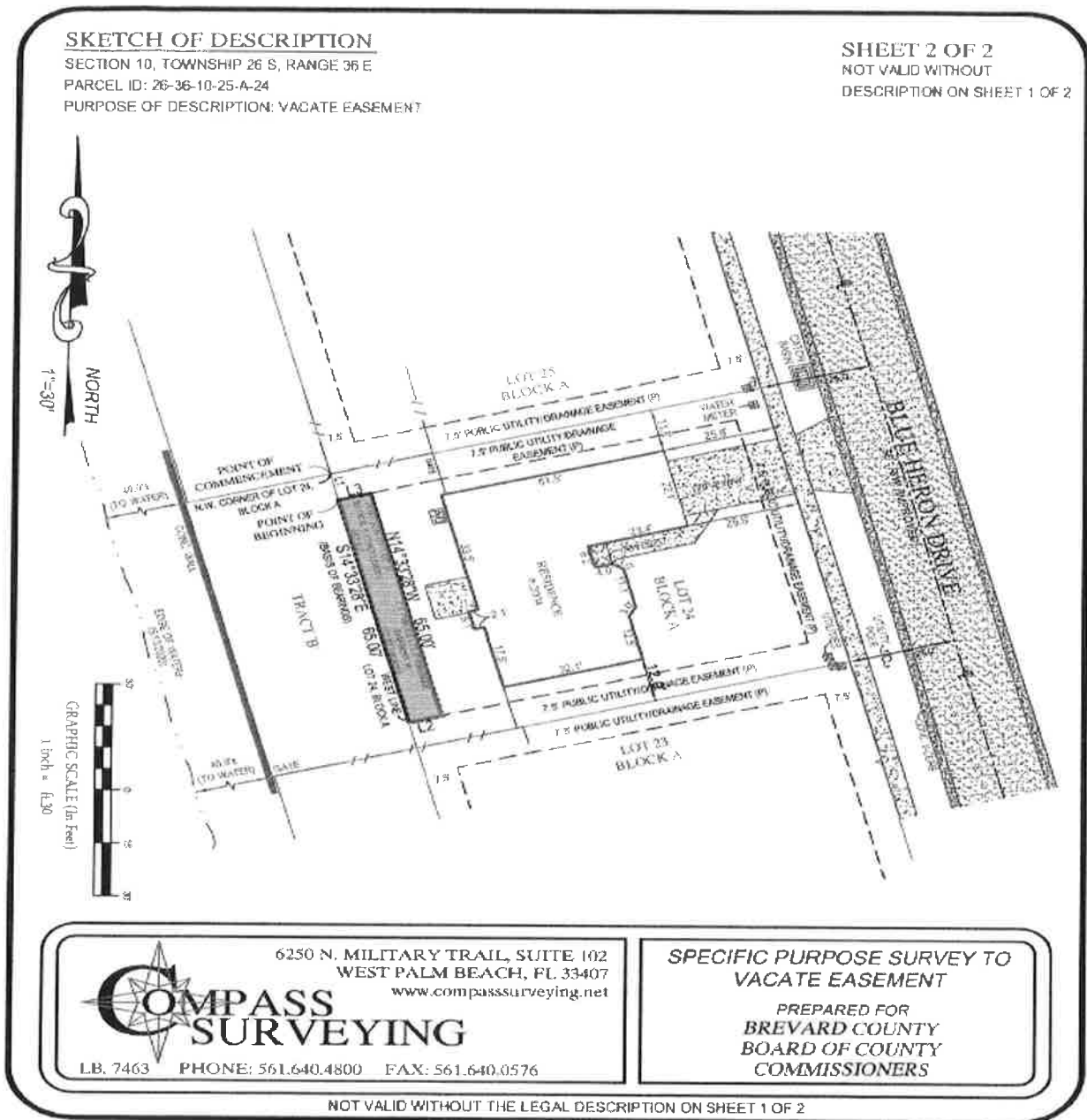
Figure 5: Sketch of description. Sheet 2 of 2. Section 10, Township 26 South, Range 36 East.
