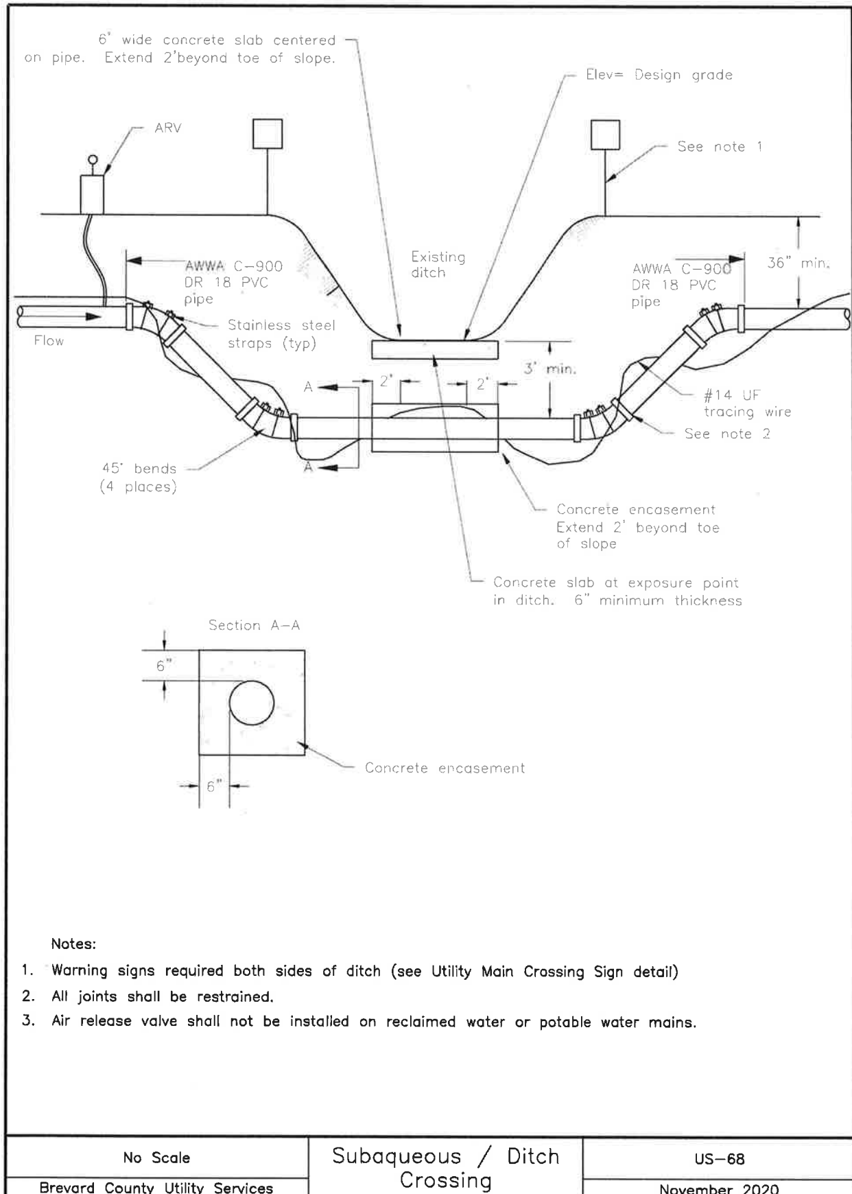
Image Description US-68 Subaqueous / Ditch Crossing
