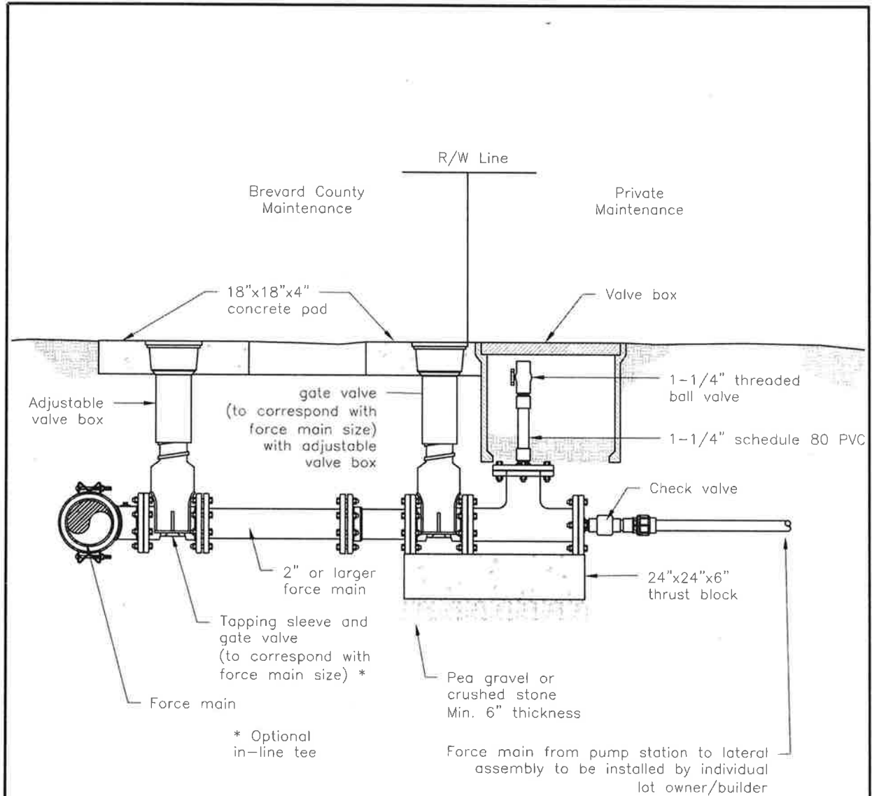
Figure 5 -Private/Public Force main Transition (US-14)
