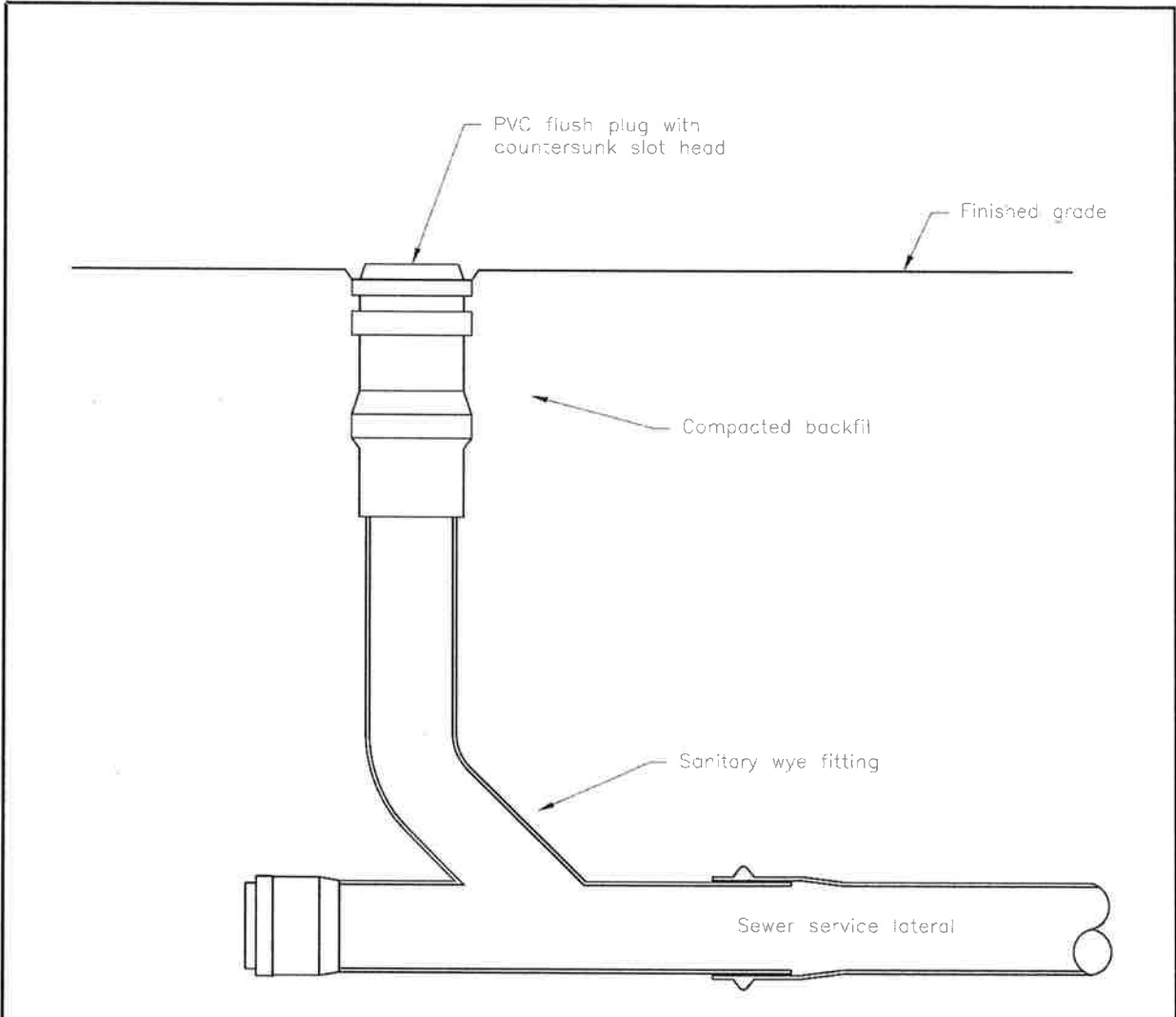
Figure 3 -Sewer Cleanout Detail (US-12)
