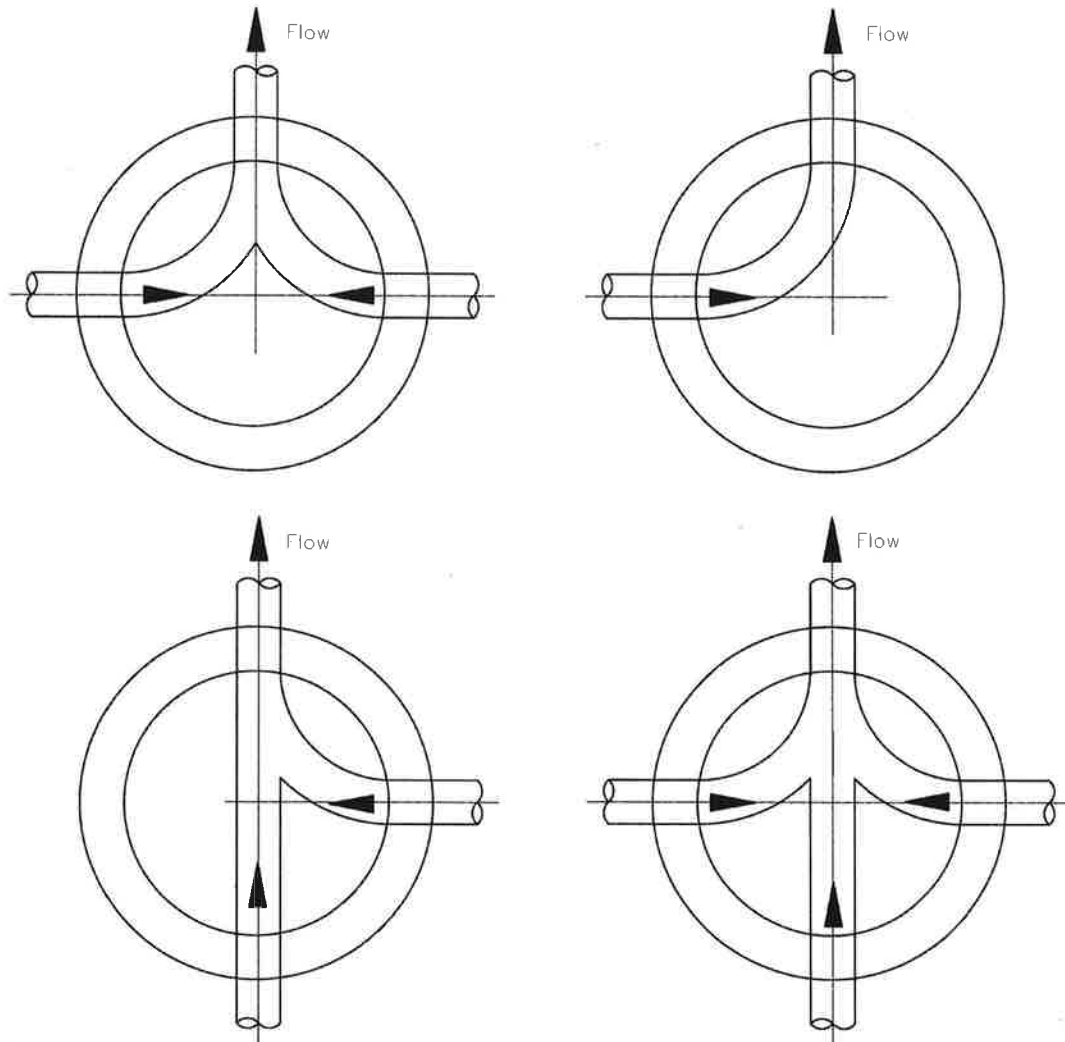
Figure 18 - Manhole Inverts Detail (US-28)
