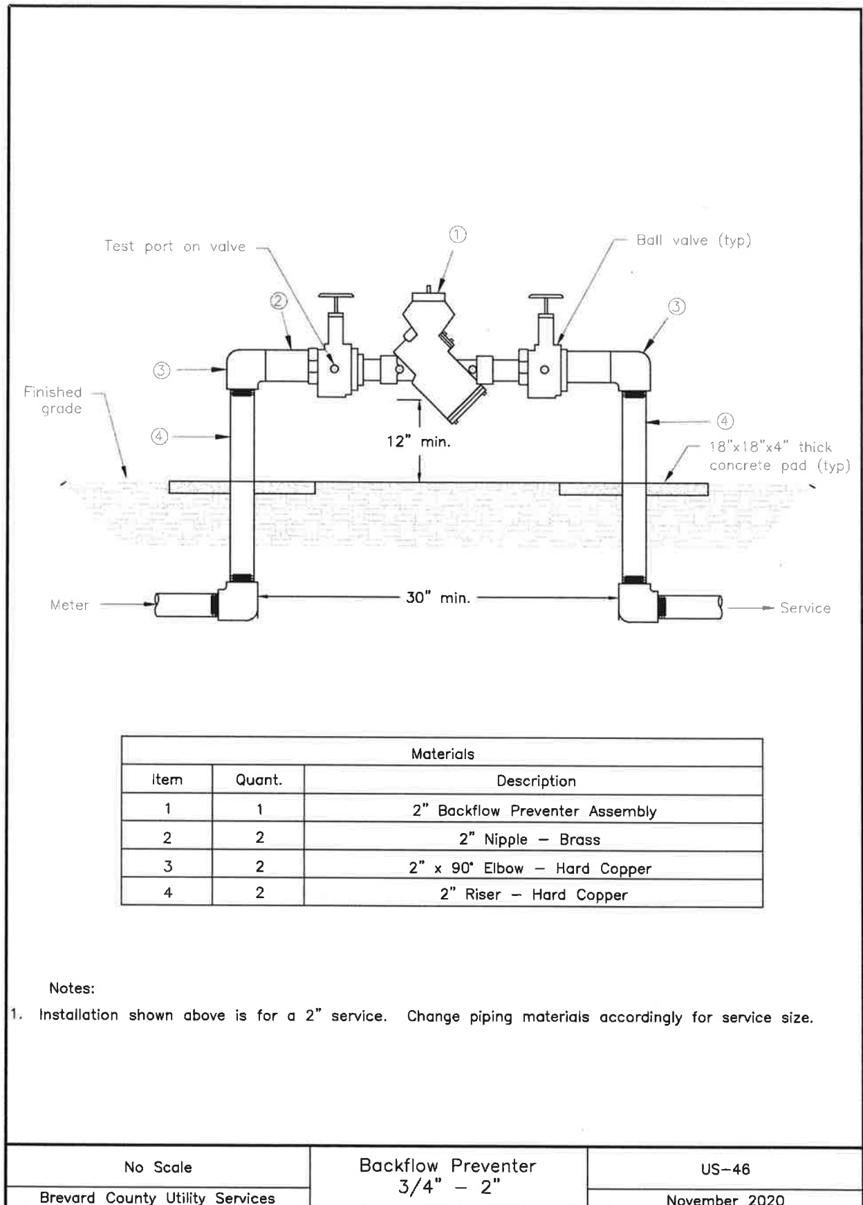
Image Description US-46 Backflow Preventer 3/4" - 2"
