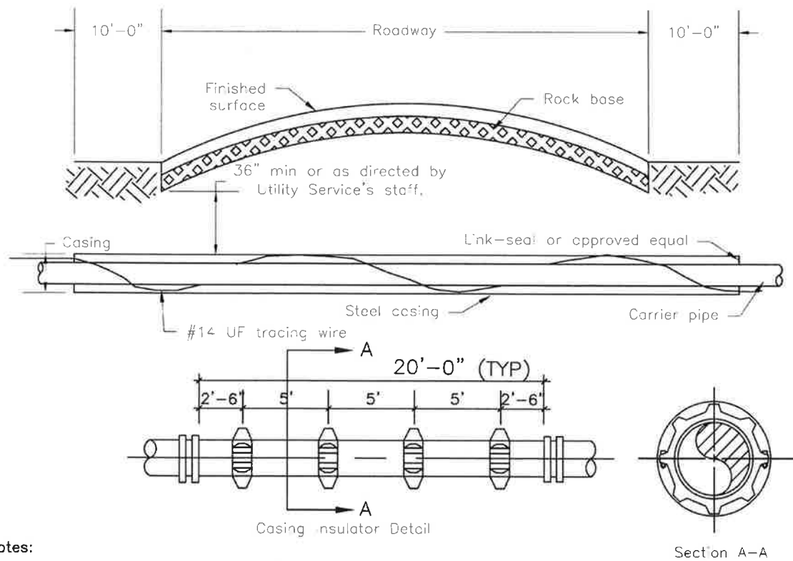
Figure 57 - Casing Installation Detail (US-70)
